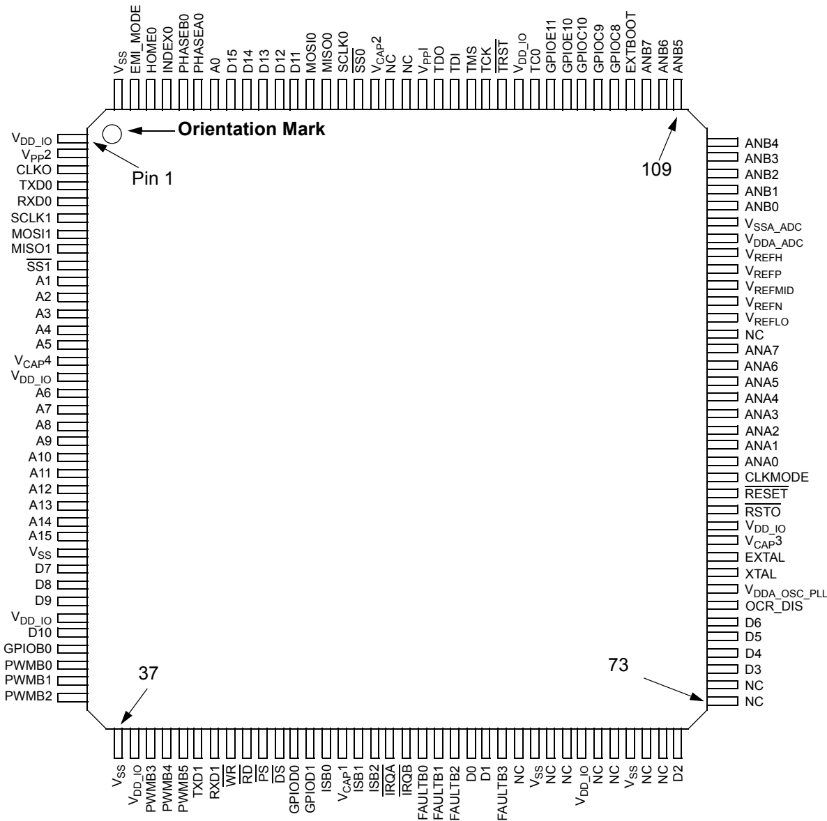
Figure 11-2 Top View, 56F8166 144-Pin LQFP Package
