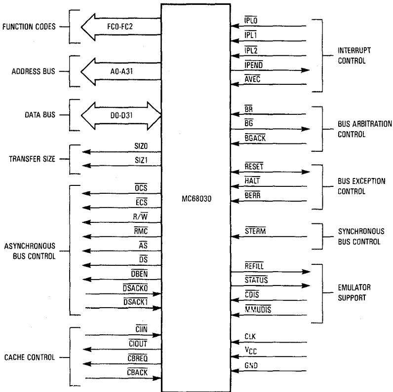
Figure 5-1. Functional Signal Groups
