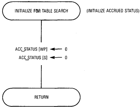
Figure 9-26. Table Search Initialization Flowchart
