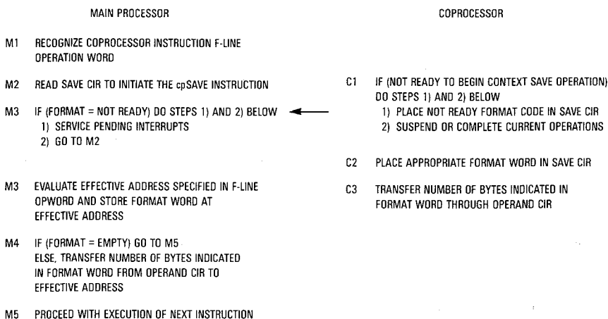
Figure 10-16. Coprocessor Context Save Instruction Protocol
