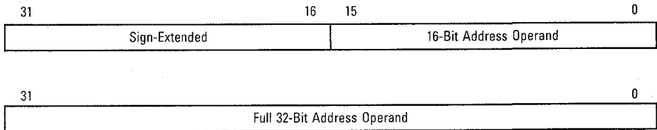
Address Organization in Address Registers
