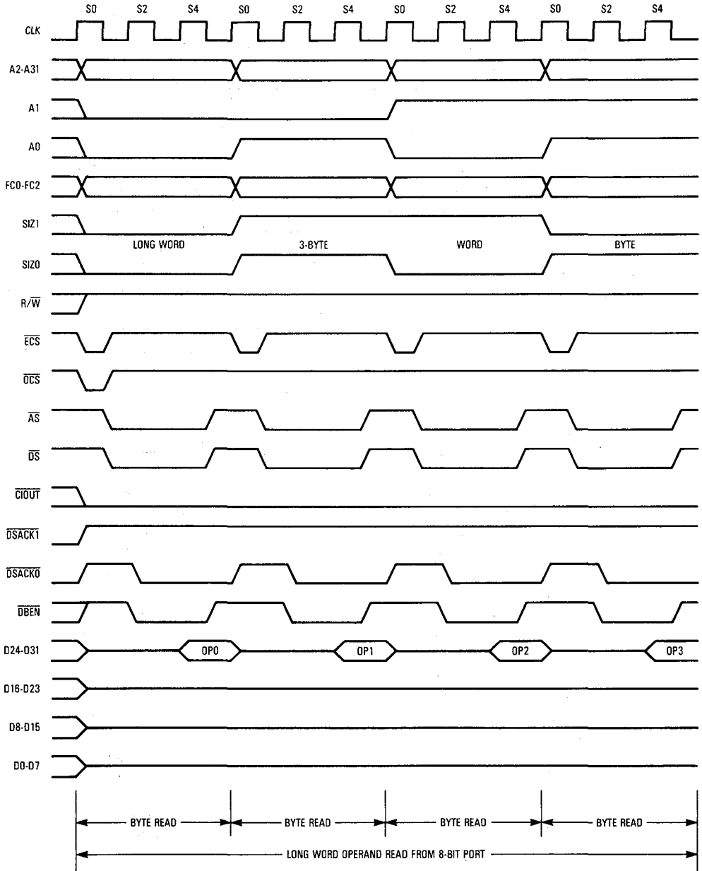
Figure 7-22. Long-Word Read — 8-Bit Port with \overline{\text{CIOUT}} Asserted
