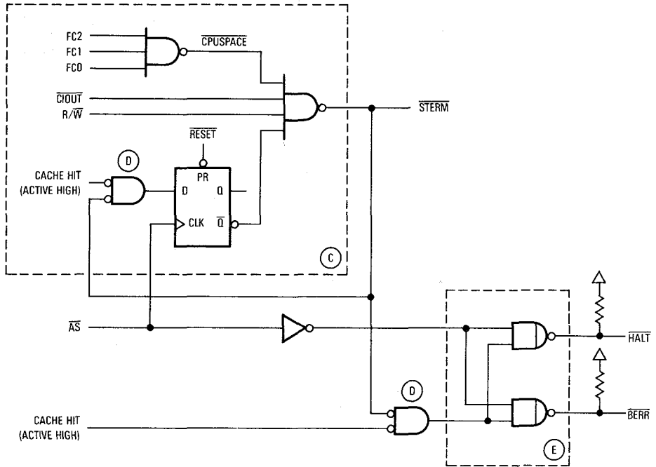
Figure 12-18. Example Early Termination Control Circuit
