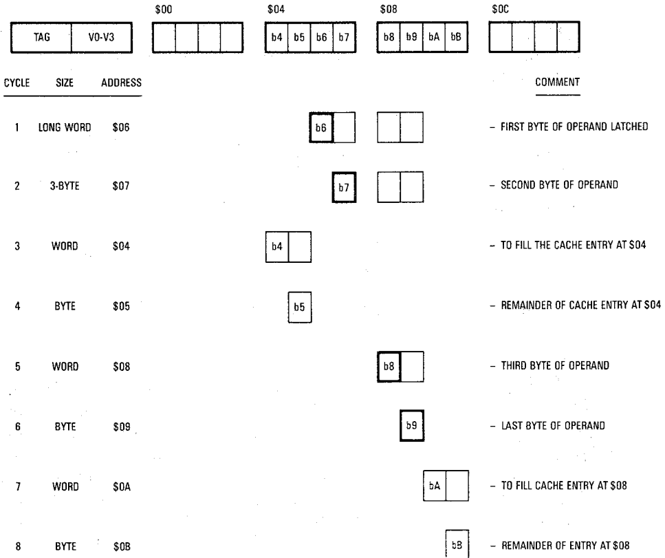
Figure 6-8. Single Entry Mode Operation — Misaligned Long Word and 8-Bit Port
