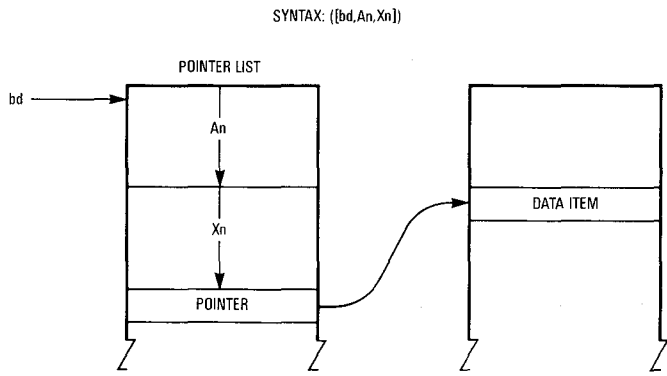
Figure 2-11. Preindexed Indirect Addressing
