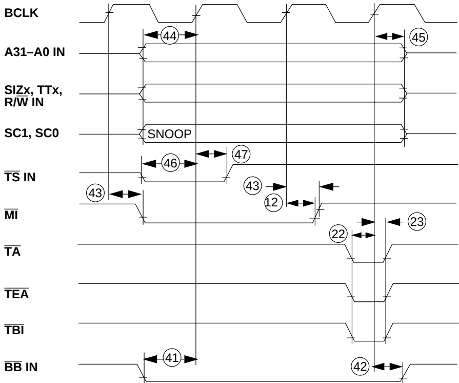
Figure B-11. Snoop Miss Timing
