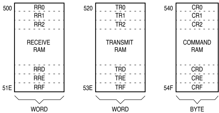
Figure 14 QSPI RAM
