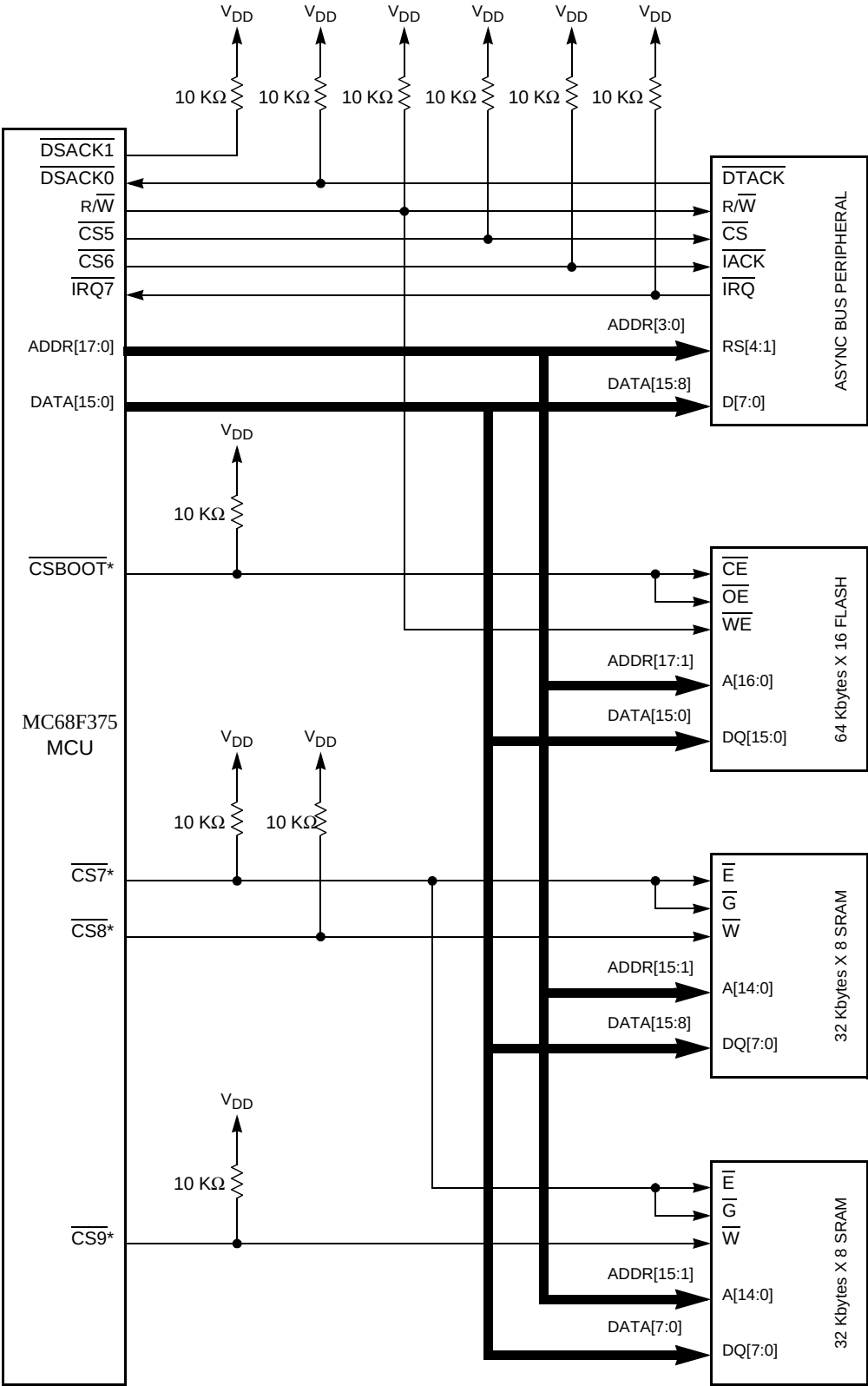
1. THESE CHIP-SELECT LINES ARE CONFIGURED FOR 16-BIT PORT OPERATION IN THIS EXAMPLE. F396 SCIM2E BUS
