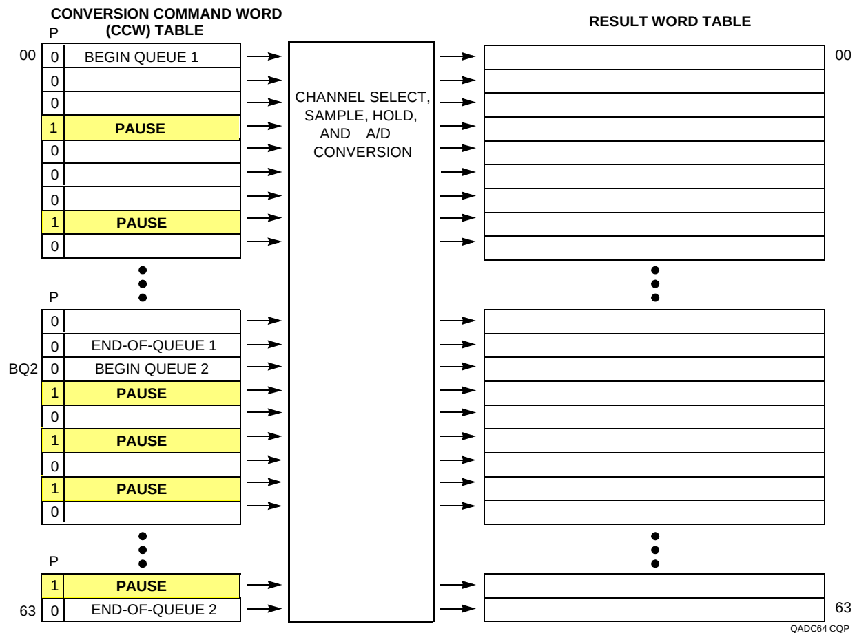
Figure 5-7 QADC64 Queue Operation with Pause
