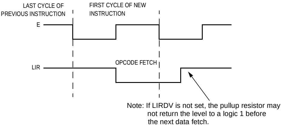
Figure 2-8. \overline{\text{LIR}} Timing
