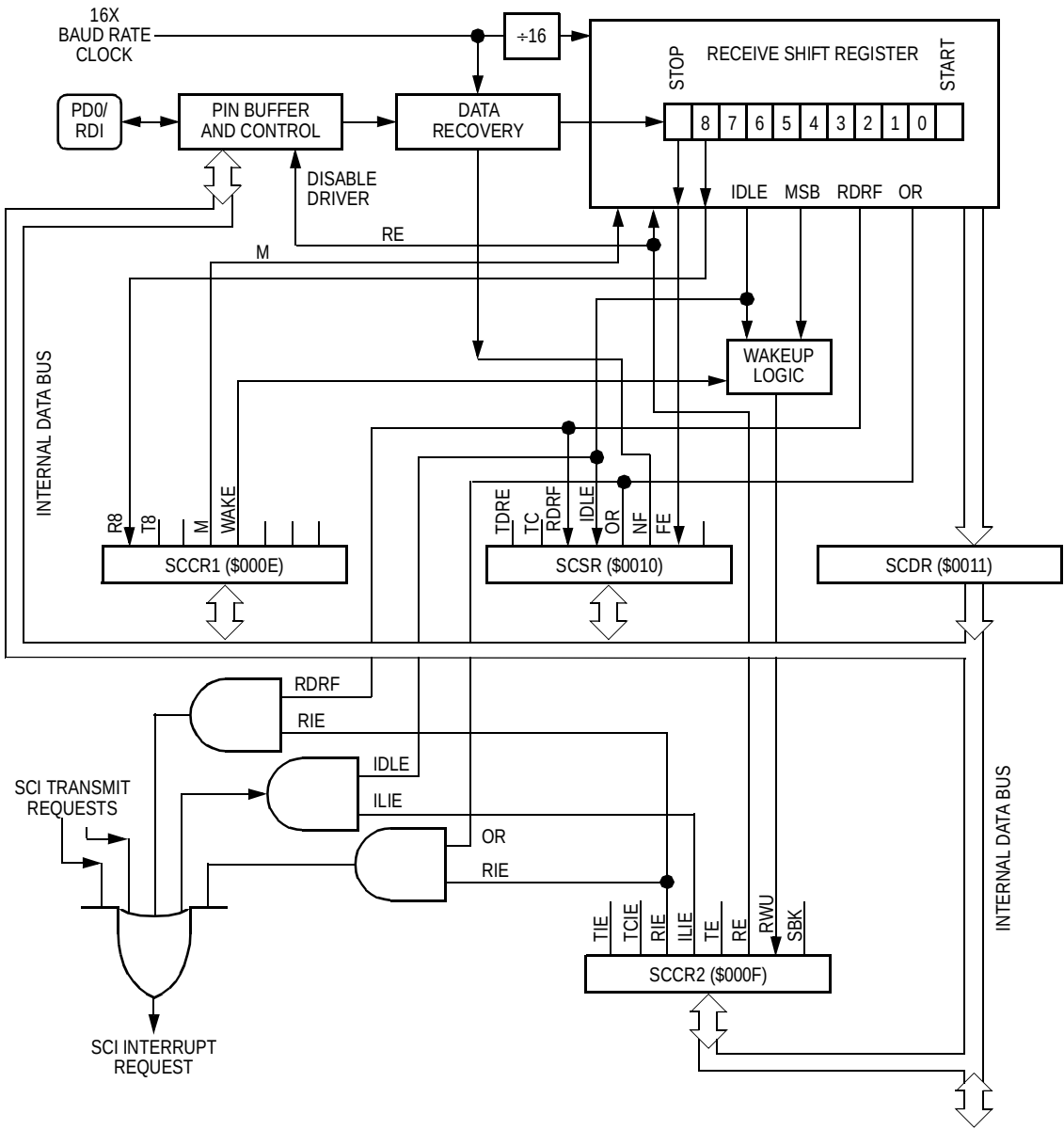
Figure 10-4. SCI Receiver
