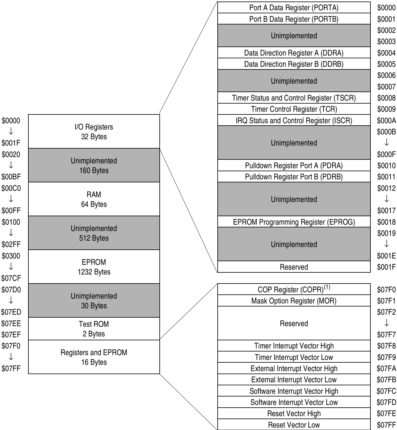
Figure 2-1. Memory Map
