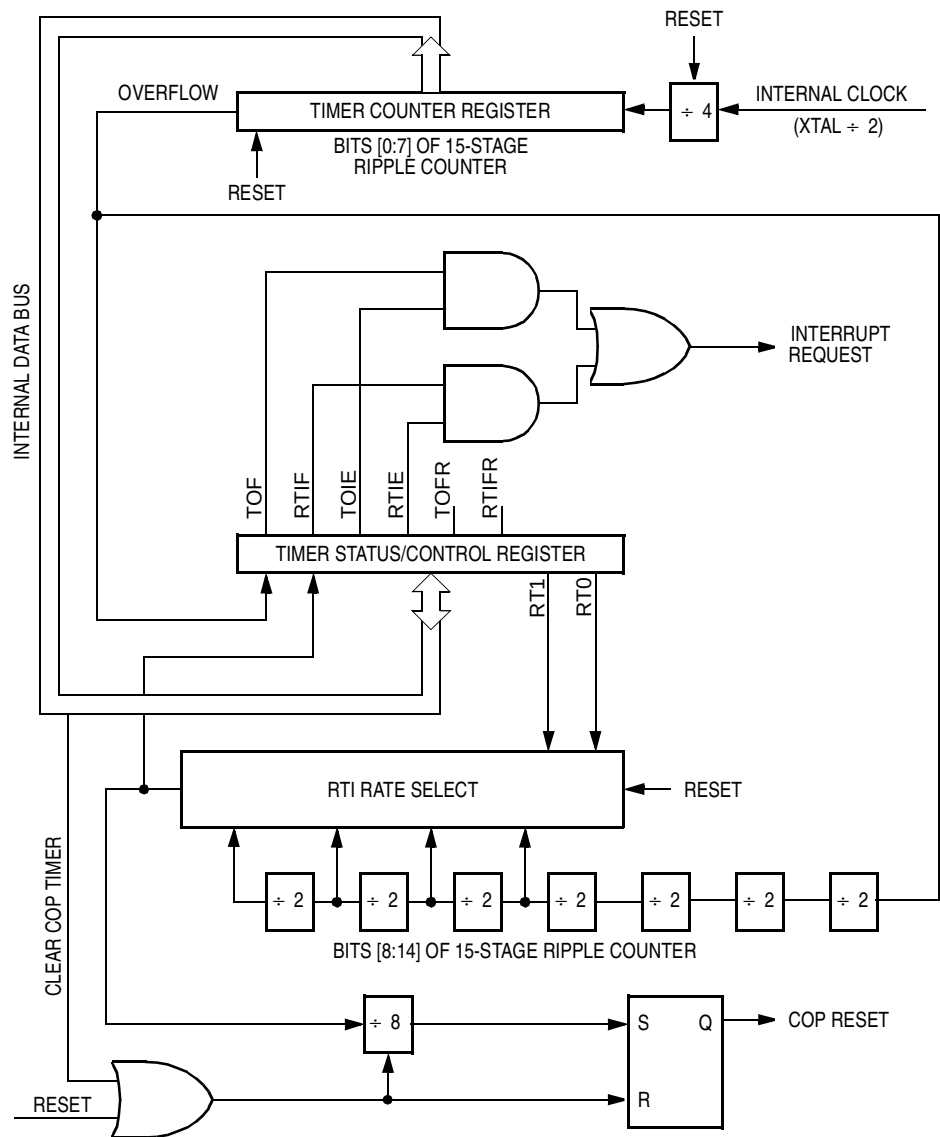
Figure 9-1. Multifunction Timer Block Diagram
