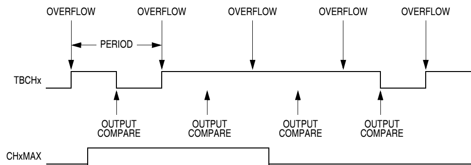
Figure 12-13. CHxMAX Latency
