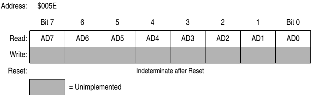
Figure 12-3. ADC Data Register (ADR)
