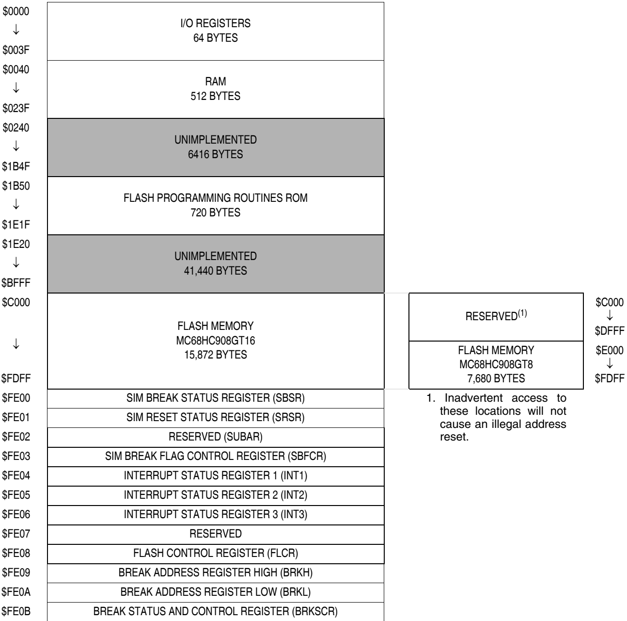
Figure 2-1. Memory Map
