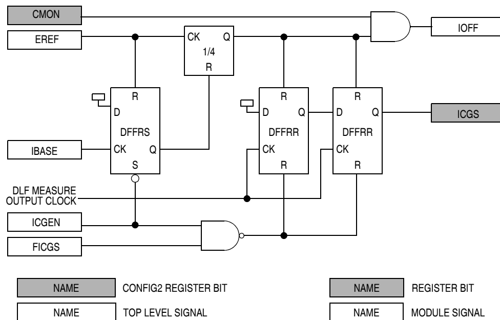
The internal clock stable bit (ICGS) is also generated in the internal clock activity detector. ICGS is set when the internal clock generator's filter stable signal (FICGS) indicates that IBASE is within about 5 percent of the target 307.2 \text{ kHz} \pm 25 \text{ percent} for two consecutive measurements. ICGS is cleared when FICGS is clear, the internal clock generator is turned off or is in stop mode (ICGEN is clear), or when IOFF is set.
