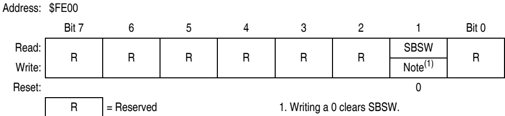
Figure 20-7. Break Status Register (BSR)
