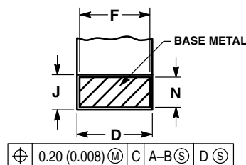
SECTION B-B VIEW ROTATED 90°
