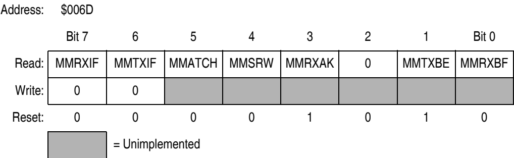
Figure 15-5. Multi-Master IIC Status Register (MMSR)
