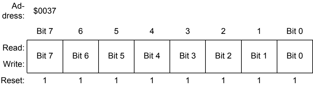
Figure 9-22. PWM Disable Mapping Write-Once Register (DISMAP)
