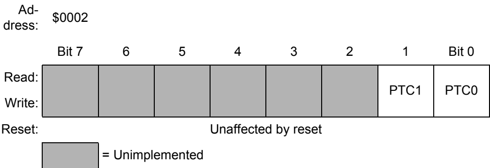
Figure 14-8. Port C Data Register (PTC)
