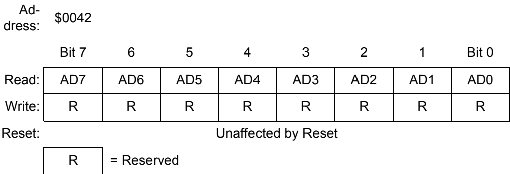
Figure 18-7. ADC Data Register Low (ADRL) Right Justified Mode
