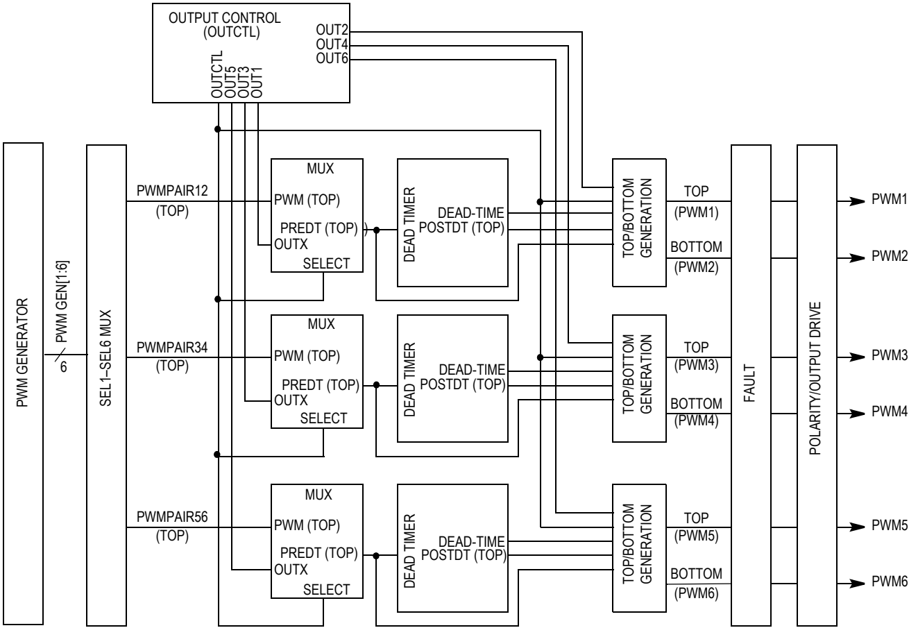
Figure 9-13. Dead-Time Generators
