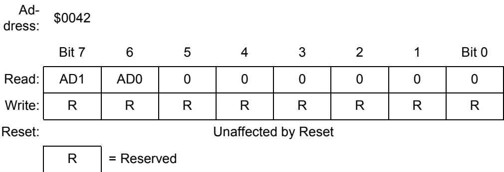
Figure 18-6. ADC Data Register Low (ADRL) Left Justified Mode
