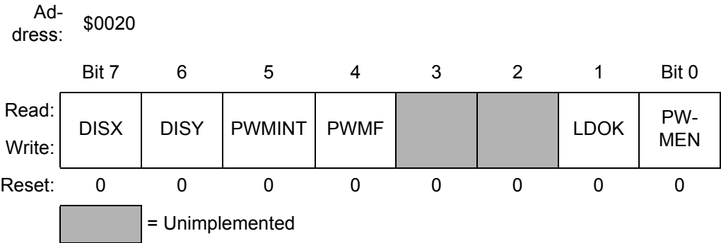
Figure 9-35. PWM Control Register 1 (PCTL1)
