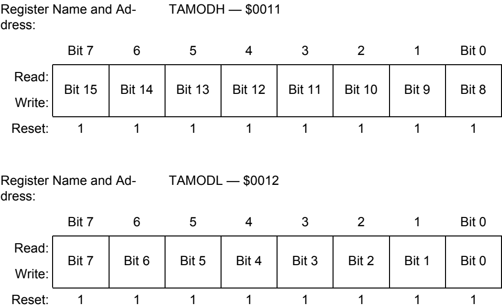
Figure 11-6. TIMA Counter Modulo Registers (TMODH and TMODL)
