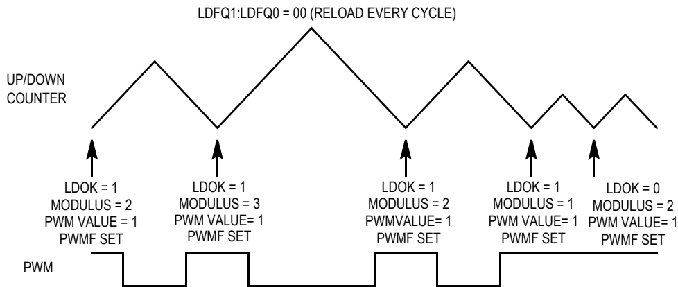
Figure 9-8. Center-Aligned Loading of Modulus
