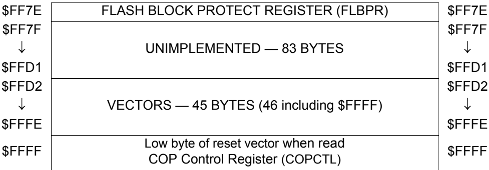
Figure 2-1. Memory Map
