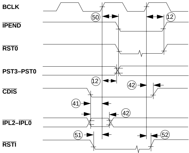
Figure B-12. Other Signal Timing
