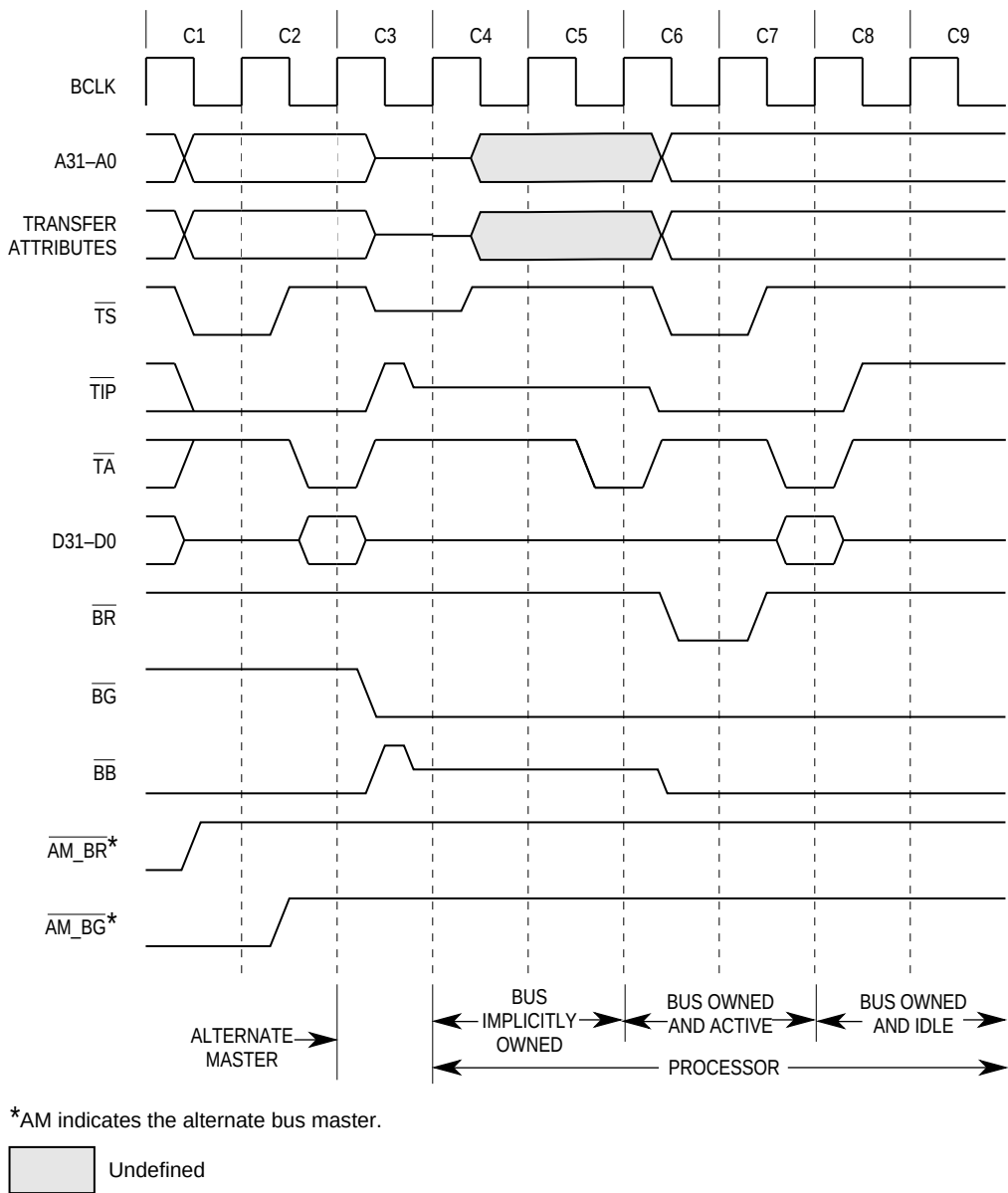
Figure 7-34. Implicit Bus Ownership Arbitration Timing
