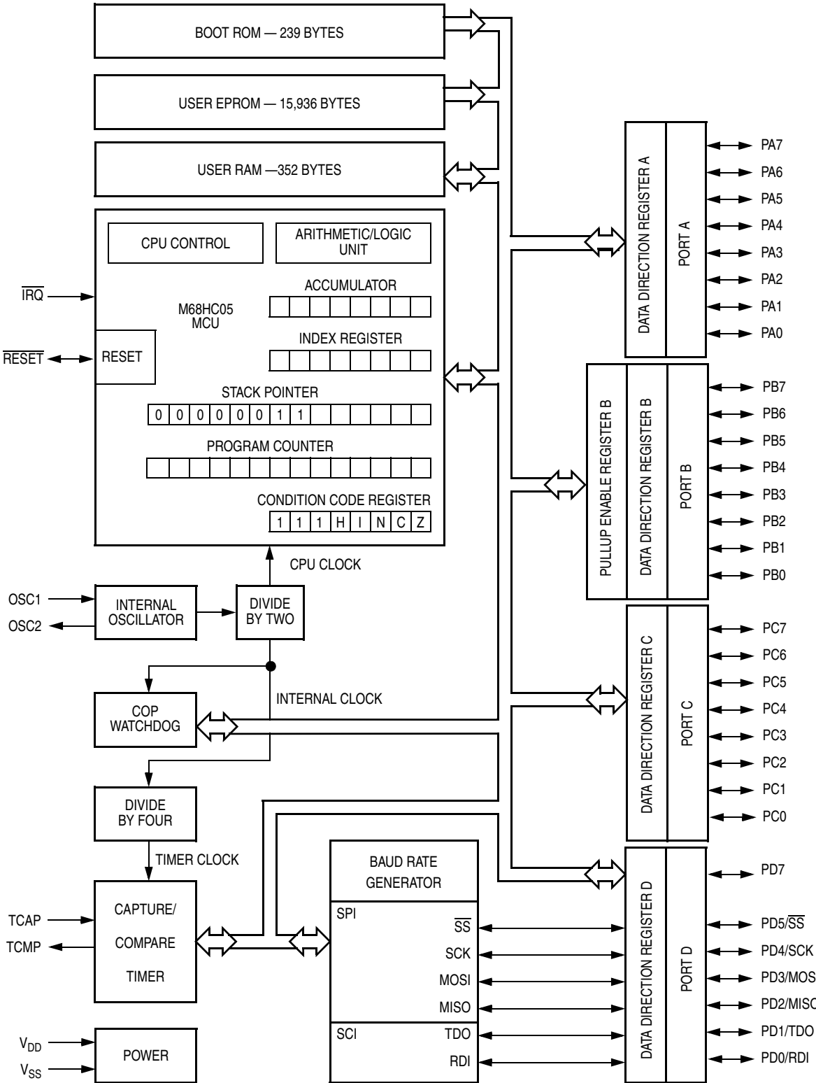
Figure 1-1. Block Diagram
