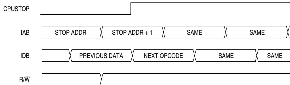
Figure 14-14. Stop Mode Entry Timing
