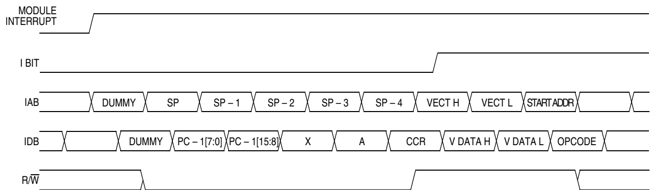
Figure 14-7. Interrupt Entry
