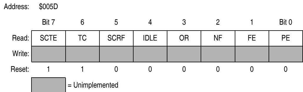
Figure 12-12. SCI Status Register 1 (SCS1)
