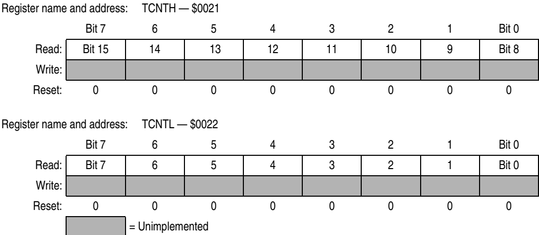
Figure 15-6. TIM Counter Registers (TCNTH and TCNTL)
