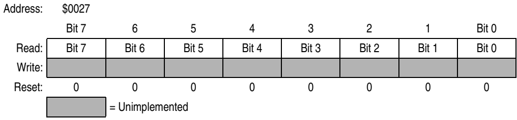
Figure 12-34. PWM Counter Register Low (PCNTL)
