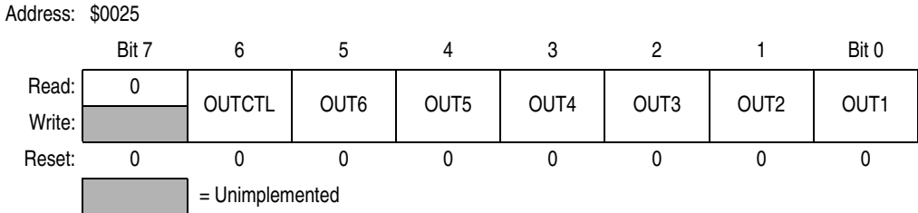
Figure 12-46. PWM Output Control Register (PWMOUT)
