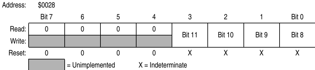
Figure 12-35. PWM Counter Modulo Register High (PMODH)
