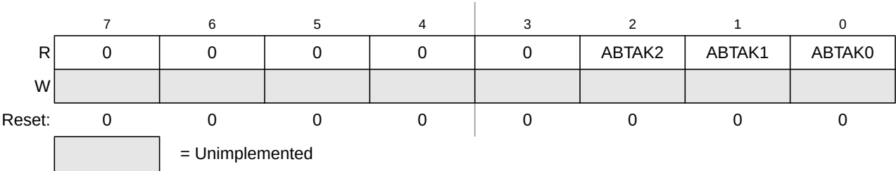
Figure 12-13. MSCAN Transmitter Message Abort Acknowledge Register (CANTAABK)
