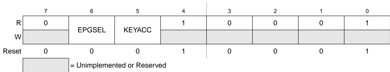
Figure 4-16. FLASH and EEPROM Configuration Register (FCNFG)
