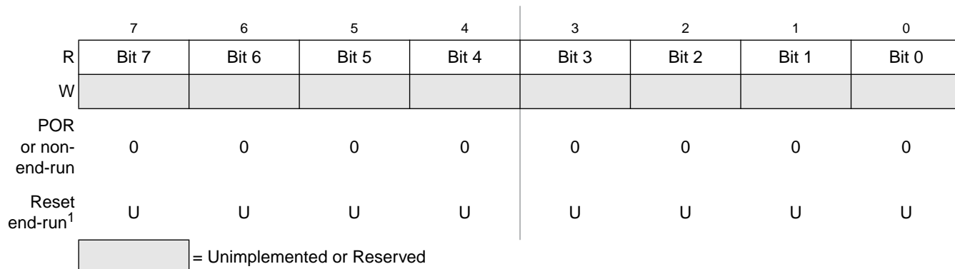
Figure 18-9. Debug FIFO Low Register (DBGFL)
