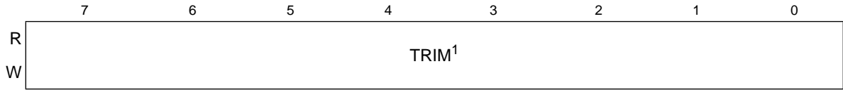
Figure 8-5. MCG Trim Register (MCGTRM)
