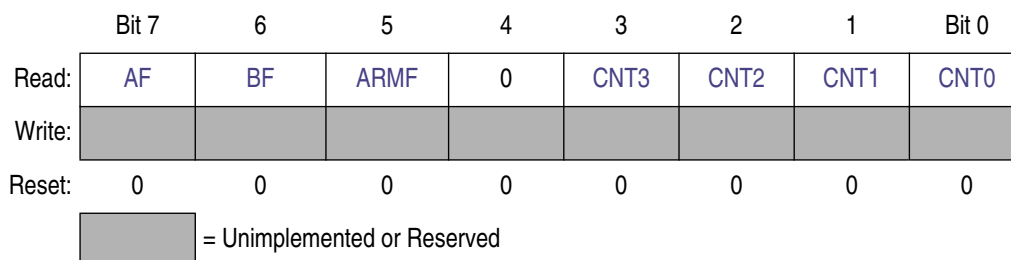
Figure 15-9. Debug Status Register (DBGS)
