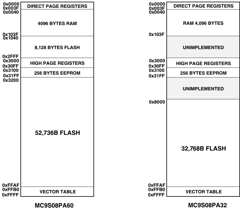
Figure 4-1. Memory map
