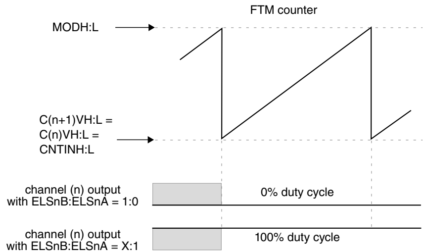
Figure 12-213. Channel (n) output if (C(n)V = C(n+1)V = CNTINH)
