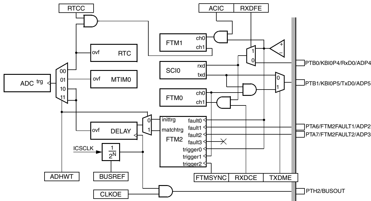
Figure 6-1. System interconnection diagram
