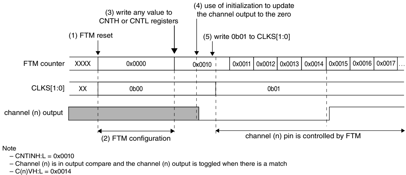
Figure 12-260. FTM behavior after the reset when the channel (n) is in output compare mode
