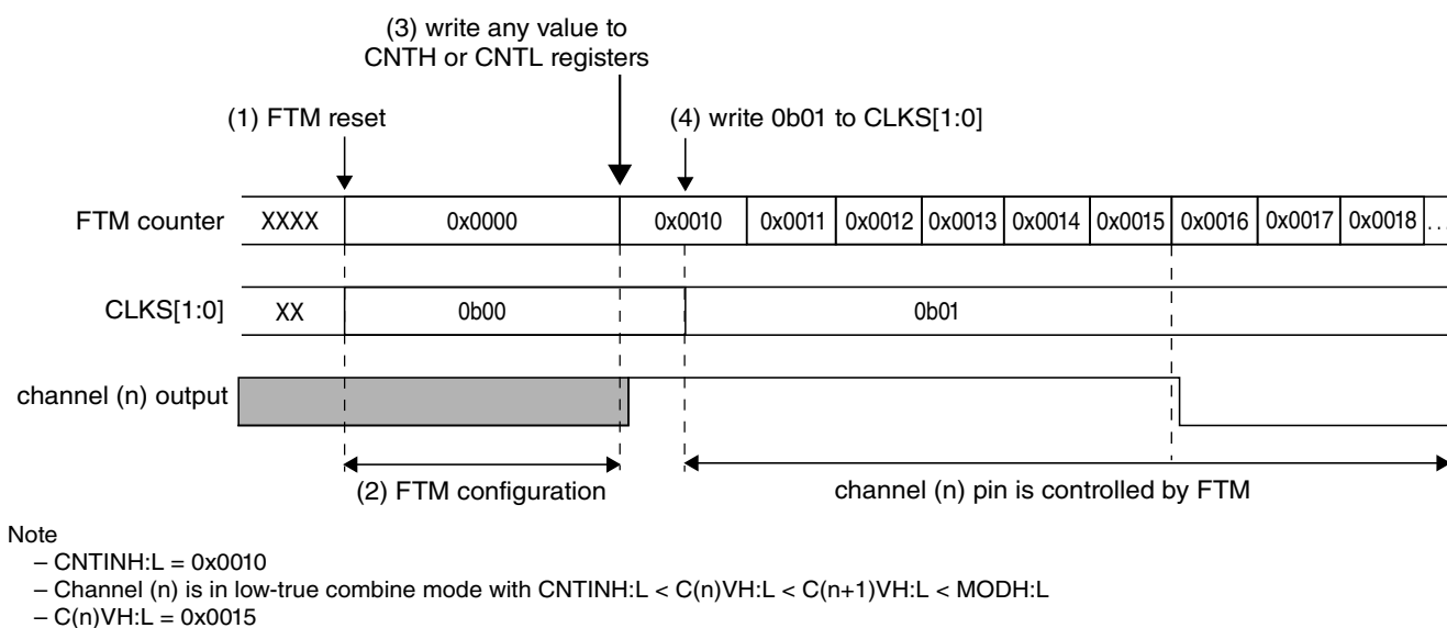
Figure 12-259. FTM behavior after the reset when the channel (n) is in combine mode
