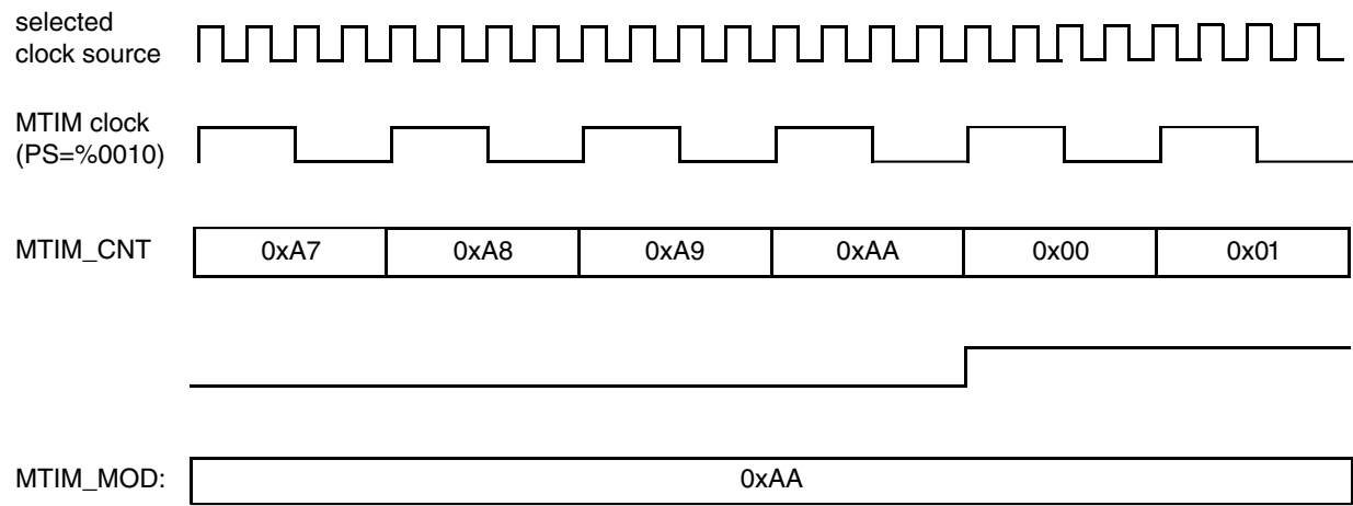
Figure 13-14. MTIM counter overflow example
