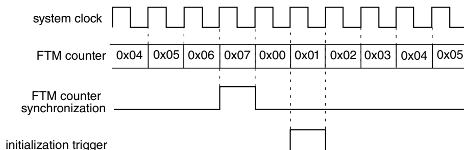
Figure 12-250. Initialization trigger is generated when there is the FTM counter synchronization
