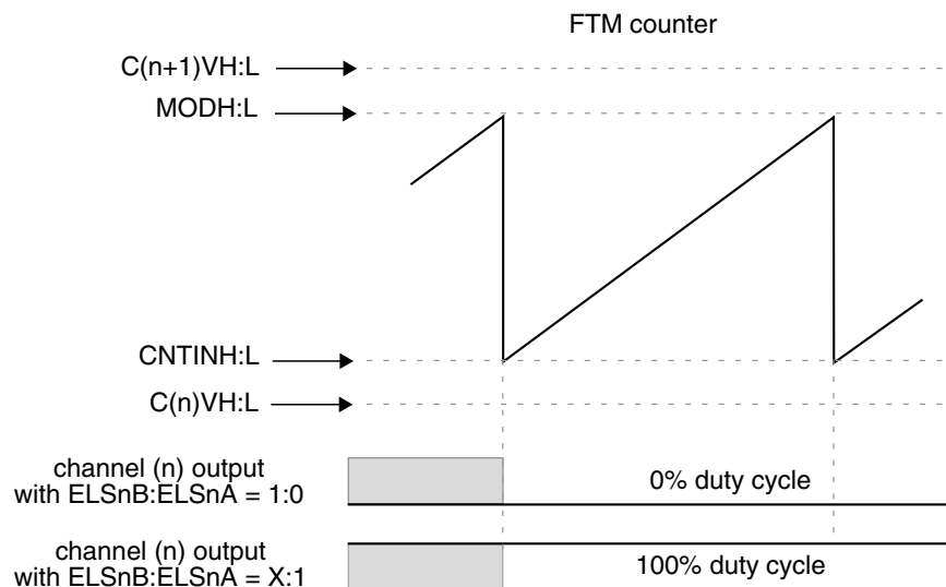
Figure 12-211. Channel (n) output if C(n)V and C(n+1)V are not between CNTIN and MOD
