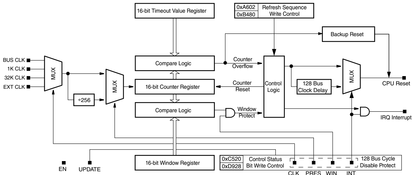
Figure 22-1. WDOG block diagram
