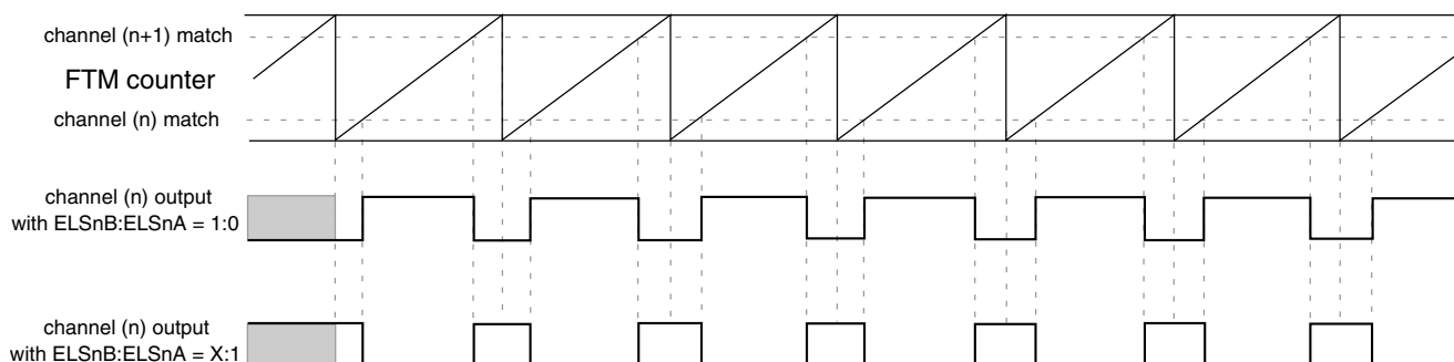
Figure 12-205. Combine mode
