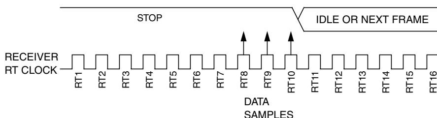
Figure 15-37. Fast data
