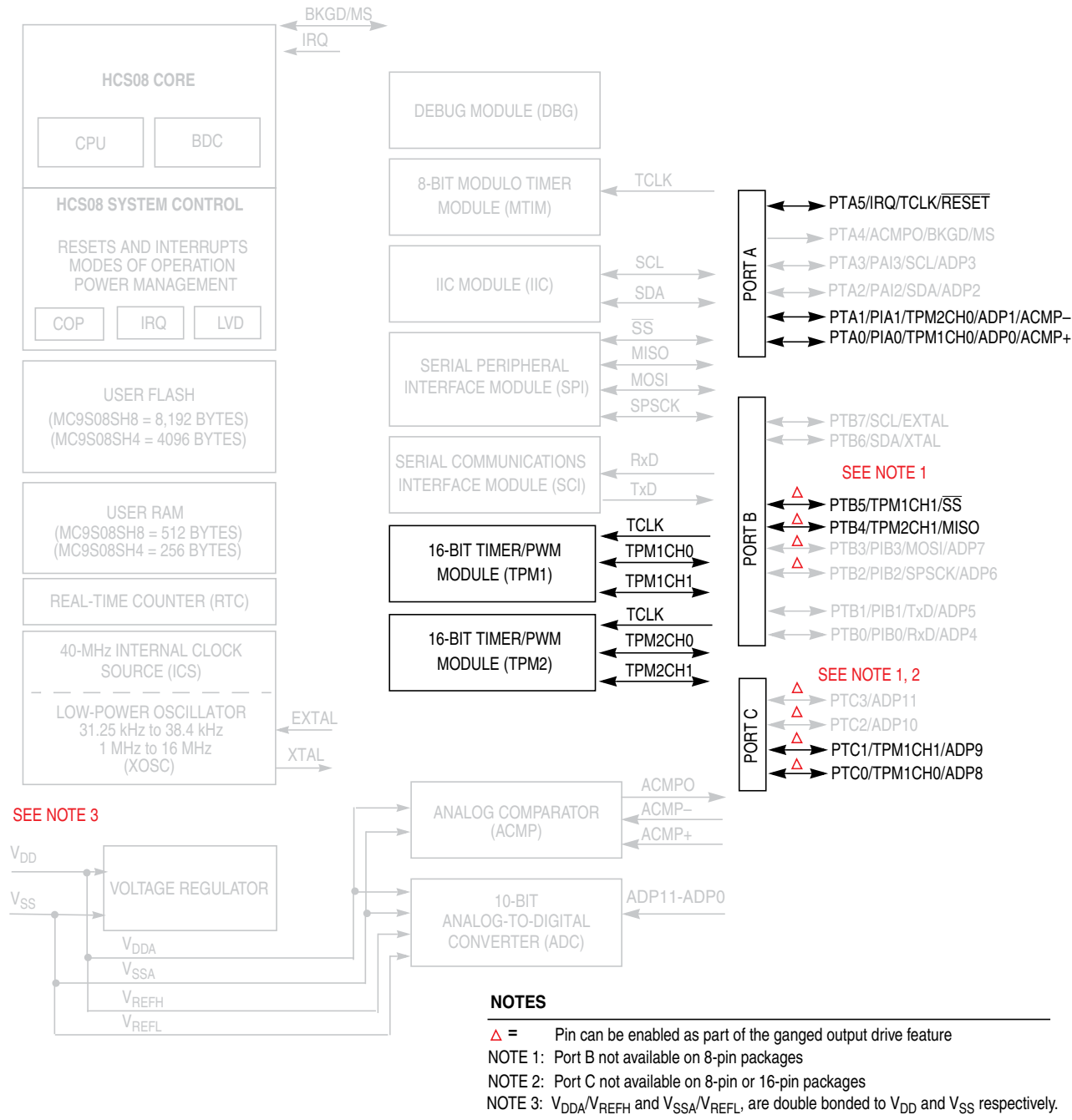
Figure 16-1. MC9S08SH8 Block Diagram Highlighting the TPM Modules
