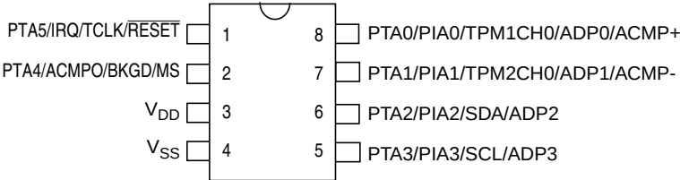
Figure 2-4. 8-Pin SOIC
