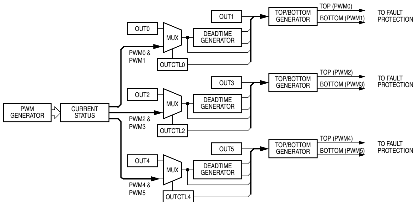
Figure 11-49. Deadtime Generators
