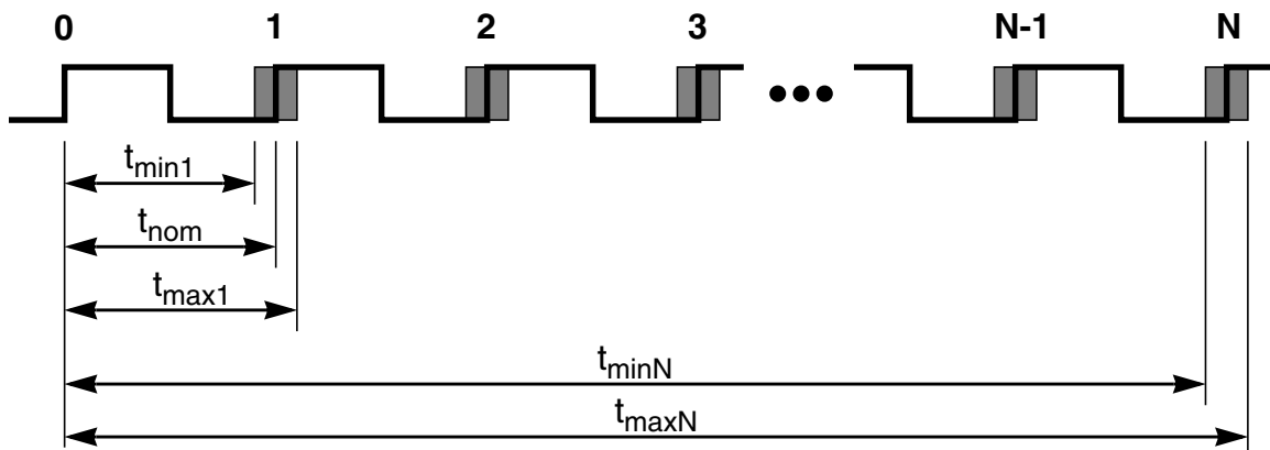
Figure 18-23. Jitter Definitions
