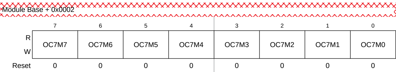
Figure 14-8. Output Compare 7 Mask Register (OC7M)
