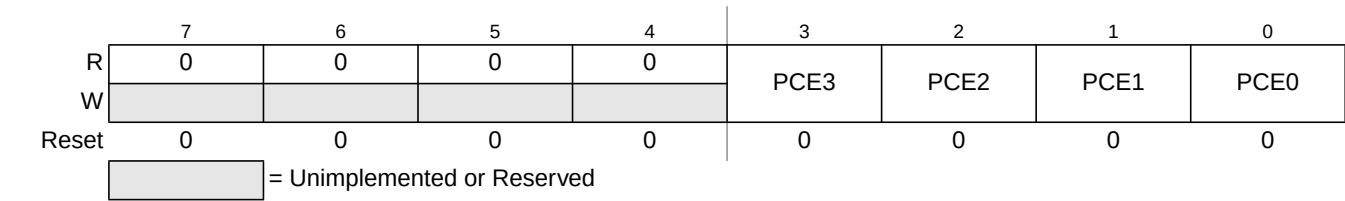
Figure 13-5. PIT Channel Enable Register (PITCE)
