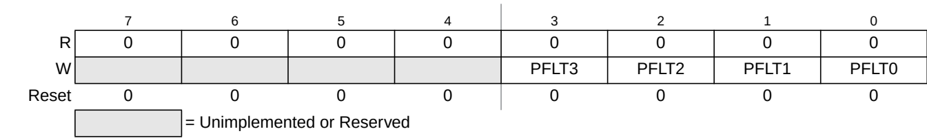
Figure 13-4. PIT Force Load Timer Register (PITFLT)
