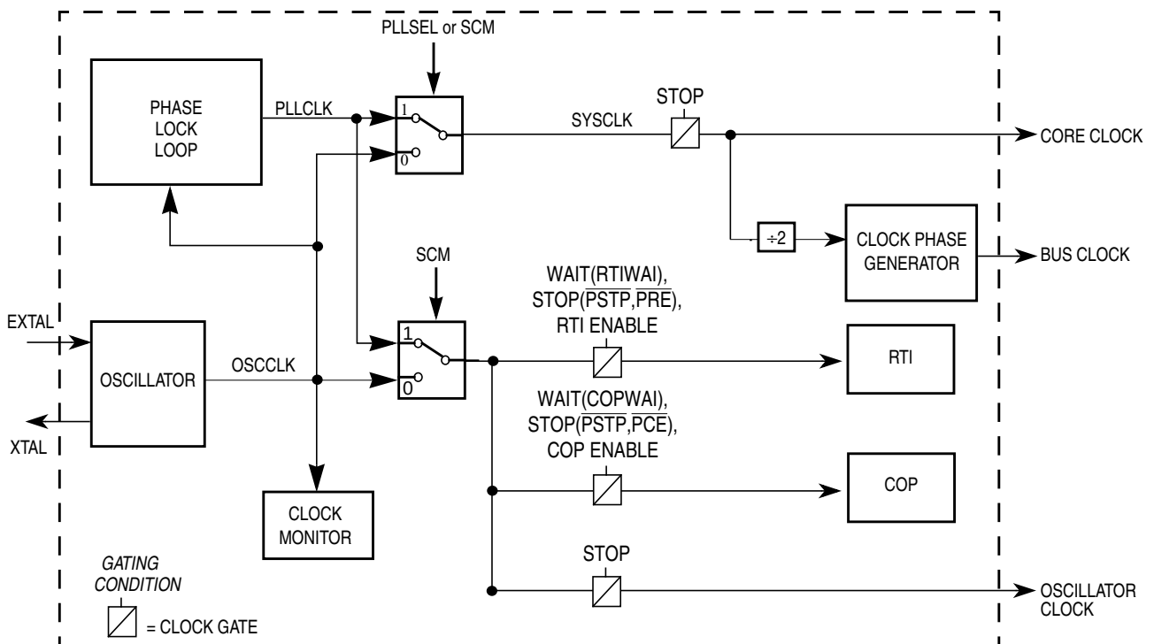
Figure 2-17. System Clocks Generator
