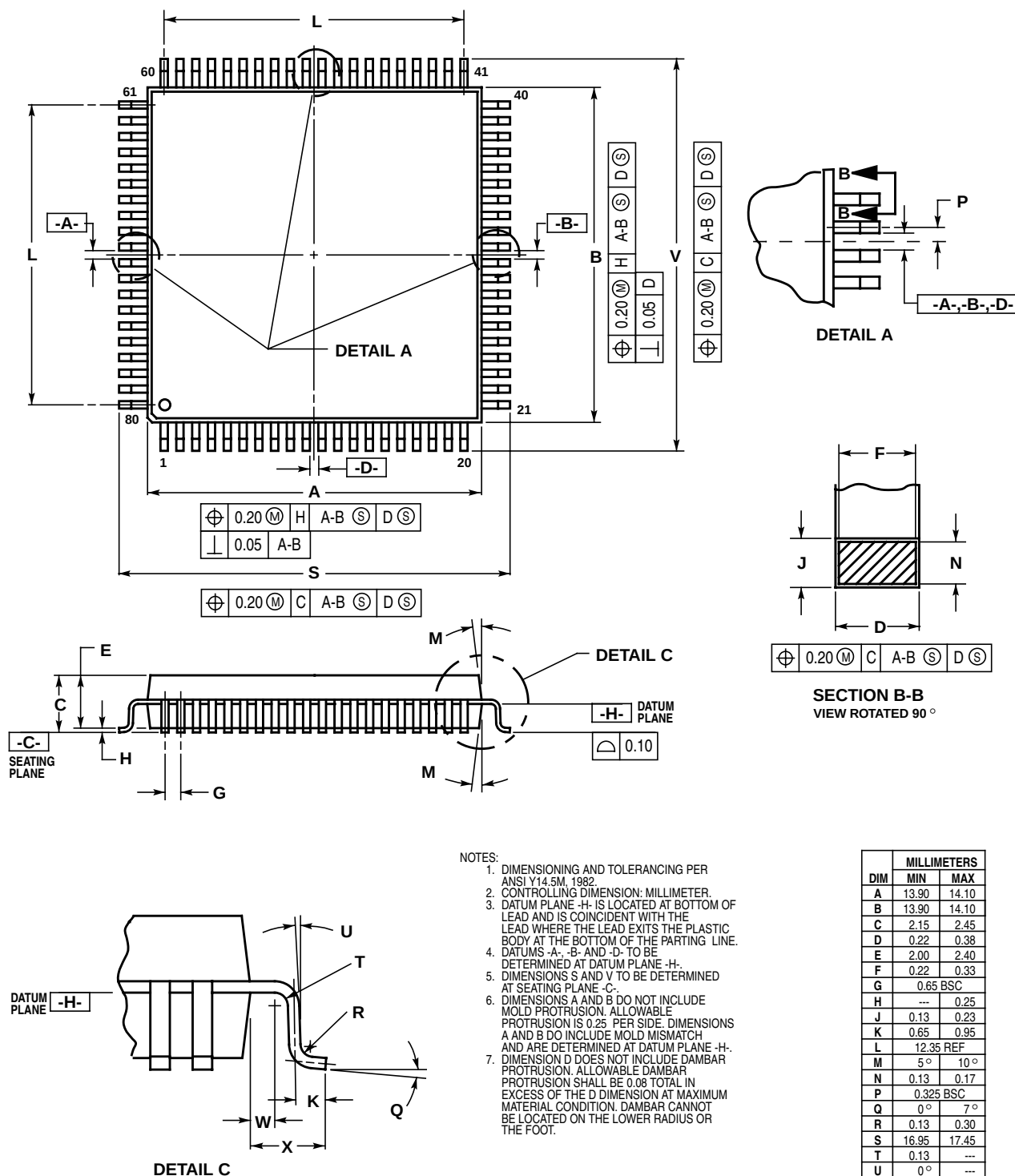
Figure B-3. 80-Pin QFP Mechanical Dimensions (Case No. 841B)
