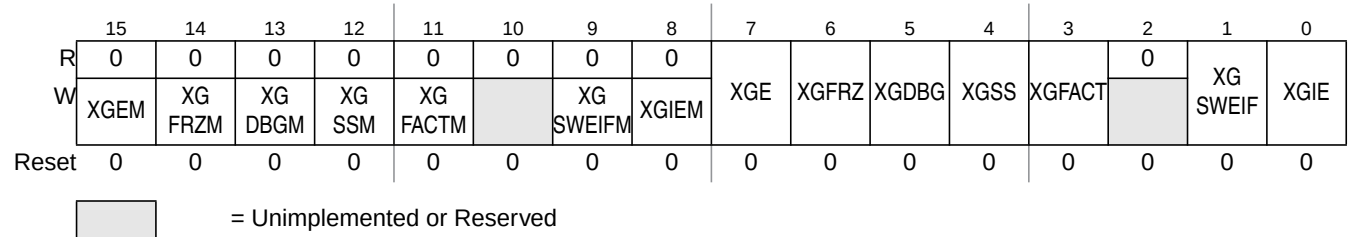
Figure 6-3. XGATE Control Register (XGMCTL)
