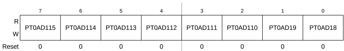
Figure 24-60. Port AD1 Data Register 0 (PT0AD1)
