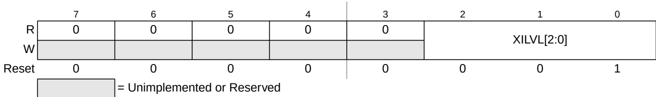
Figure 16-4. XGATE Interrupt Priority Configuration Register (INT_XGPRI0)
