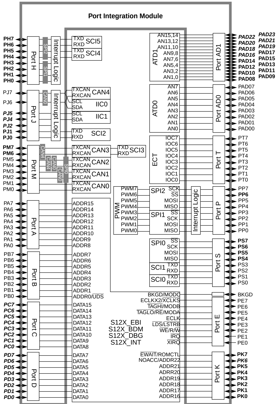
Figure 22-1. PIM Block Diagram
