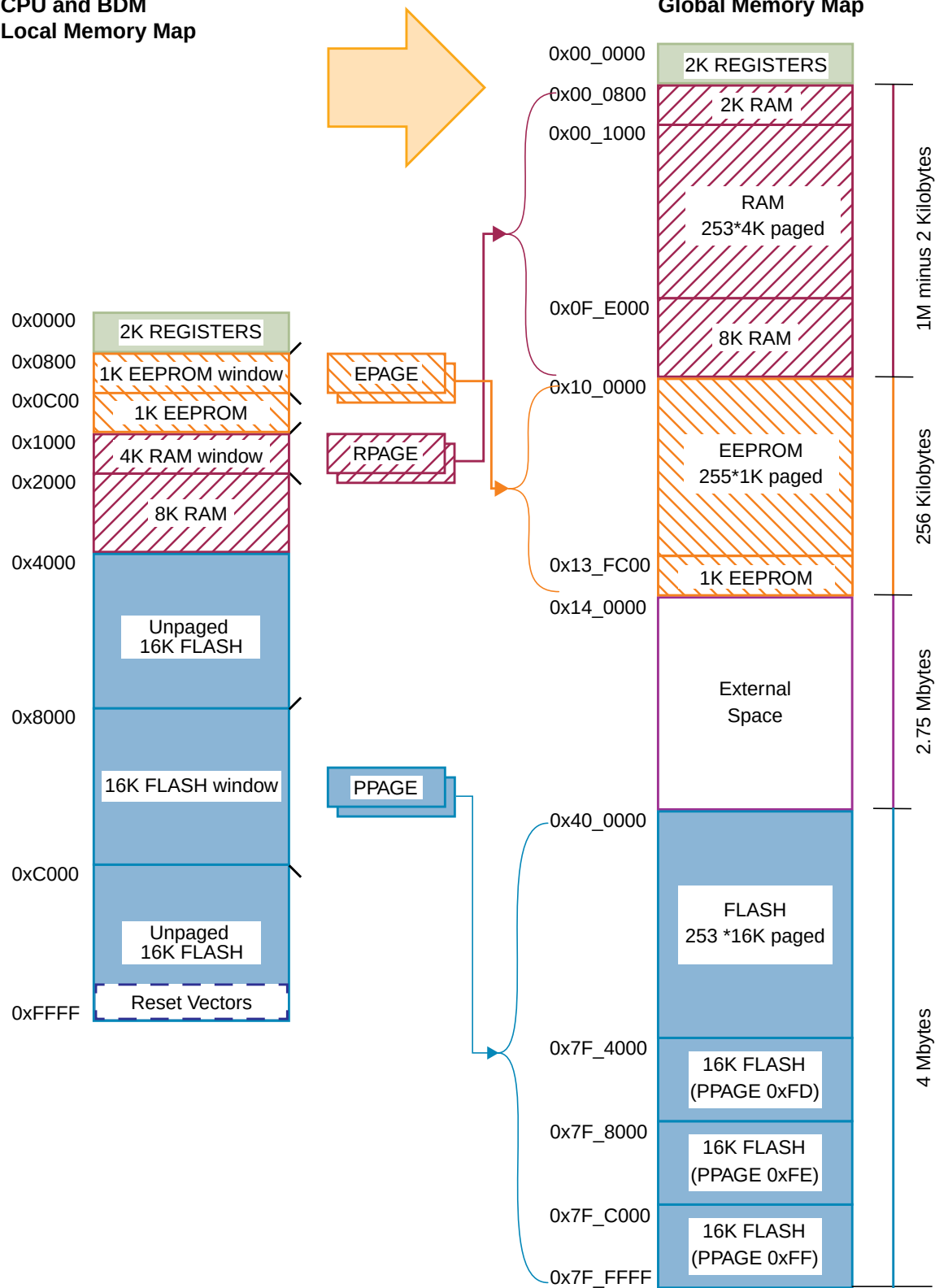
Figure 18-21. Expansion of the Local Address Map
