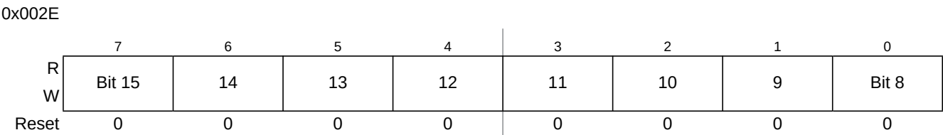
Figure 19-20. Debug Comparator Data High Mask Register (DBGXDHM)
