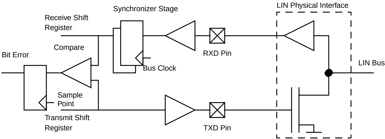
Figure 11-18. Collision Detect Principle
