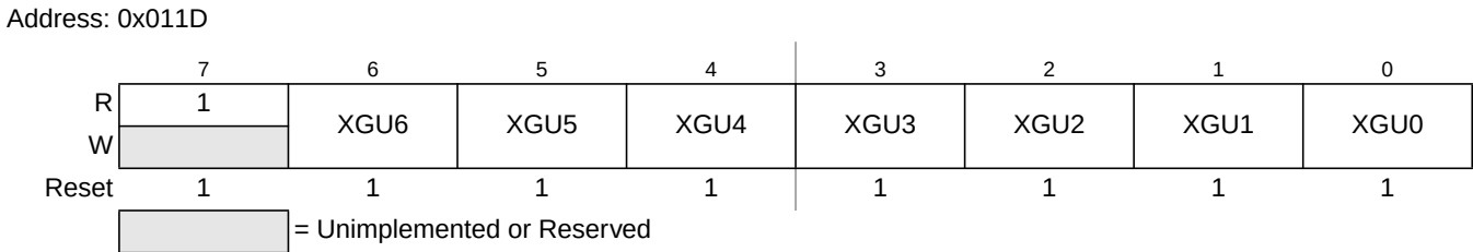
Figure 17-18. RAM XGATE Upper Boundary Register (RAMXGU)
