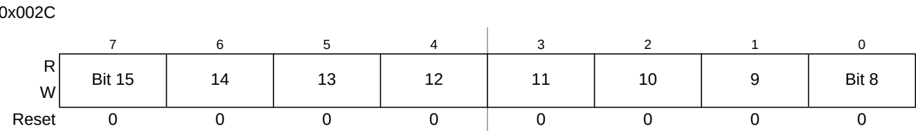
Figure 19-18. Debug Comparator Data High Register (DBGXDH)
