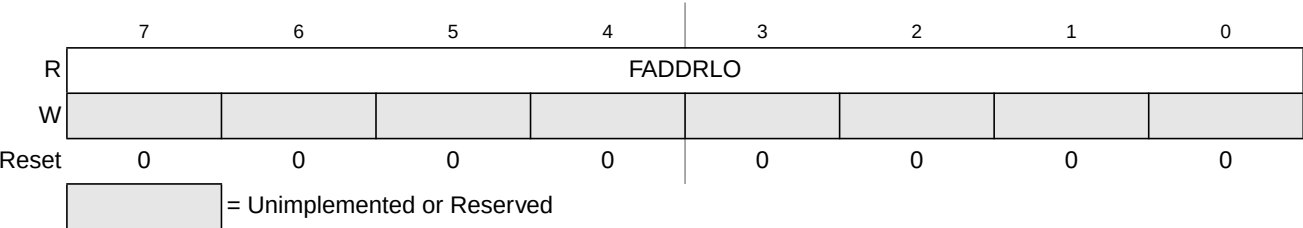
Figure 27-17. Flash Address Low Register (FADDRLO)
