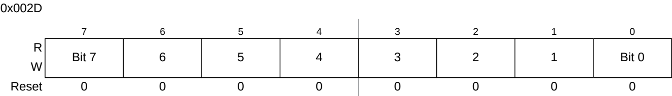
Figure 19-19. Debug Comparator Data Low Register (DBGXDL)
