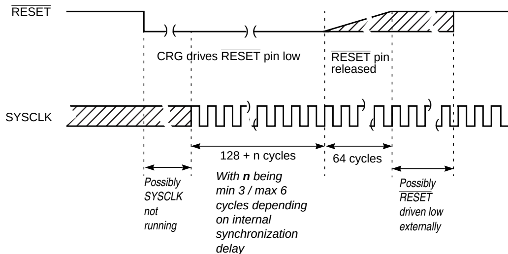
Figure 2-25. RESET Timing
