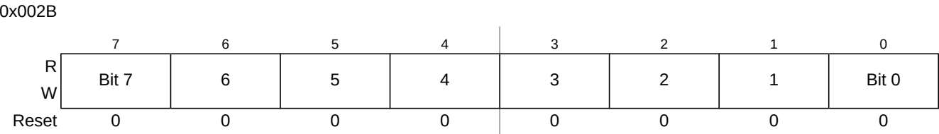
Figure 19-17. Debug Comparator Address Low Register (DBGXAL)
