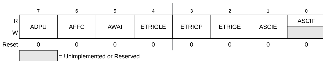
Figure 4-5. ATD Control Register 2 (ATDCTL2)
