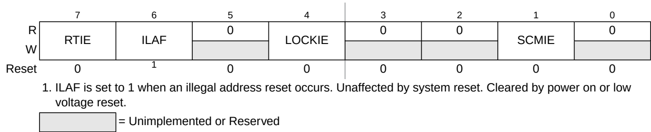
Figure 2-8. CRG Interrupt Enable Register (CRGINT)
