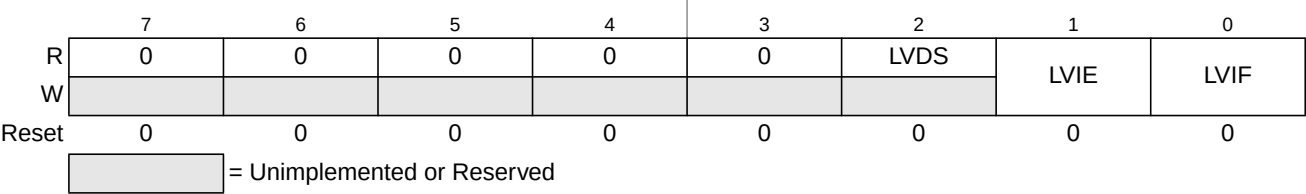
Figure 14-3. Control Register (VREGCTRL)
