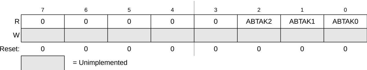
Figure 10-13. MSCAN Transmitter Message Abort Acknowledge Register (CANTAABK)
