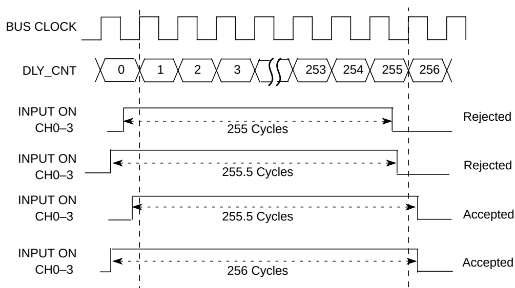
Figure 7-72. Channel Input Validity with Delay Counter Feature
