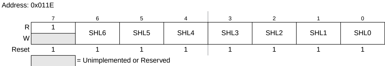
Figure 17-19. RAM Shared Region Lower Boundary Register (RAMSHL)
