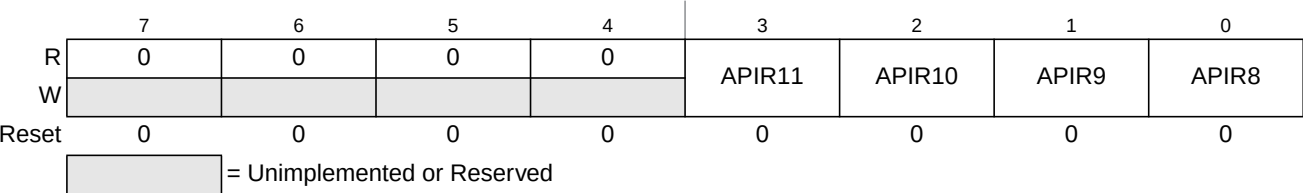
Figure 14-6. Autonomous Periodical Interrupt Rate High Register (VREGAPIRH)
