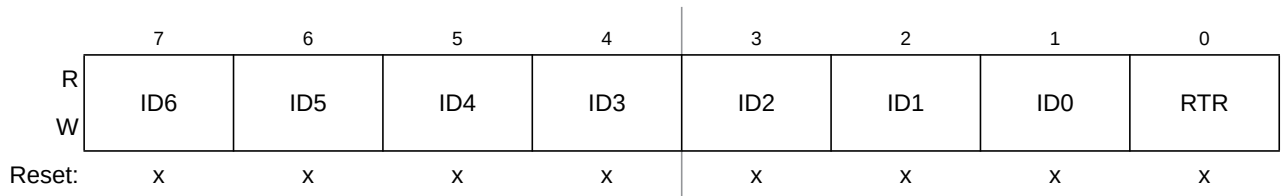
Figure 10-29. Identifier Register 3 (IDR3) — Extended Identifier Mapping
