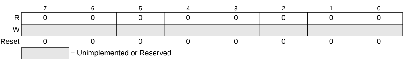
Figure 14-2. HT Control Register (VREGHTCL)
