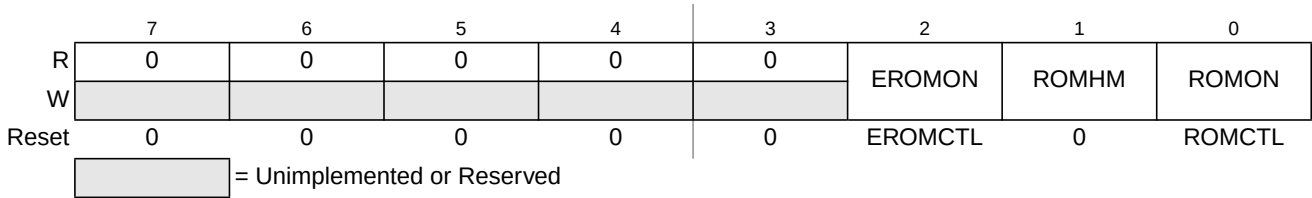
Figure 18-10. MMC Control Register (MMCCTL1)
