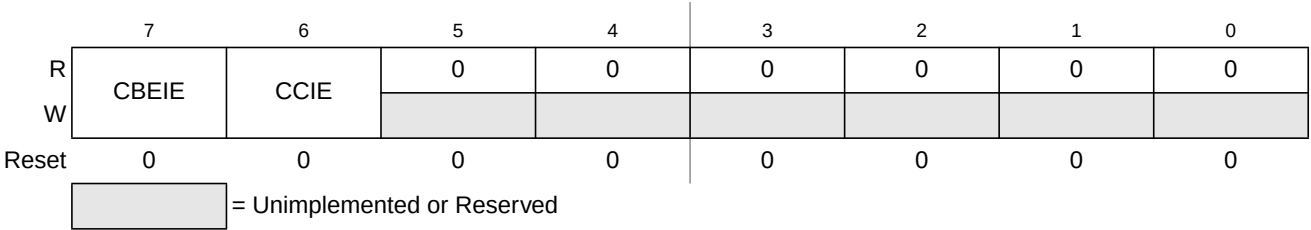
Figure 25-7. EEPROM Configuration Register (ECNFG)
