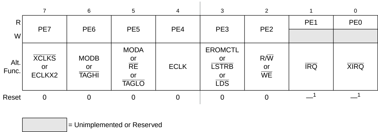
Figure 22-11. Port E Data Register (PORTE)
