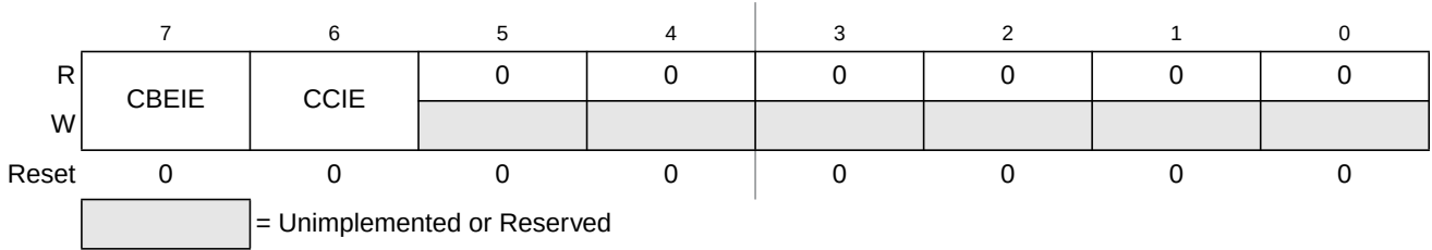
Figure 26-7. EEPROM Configuration Register (ECNFG)
