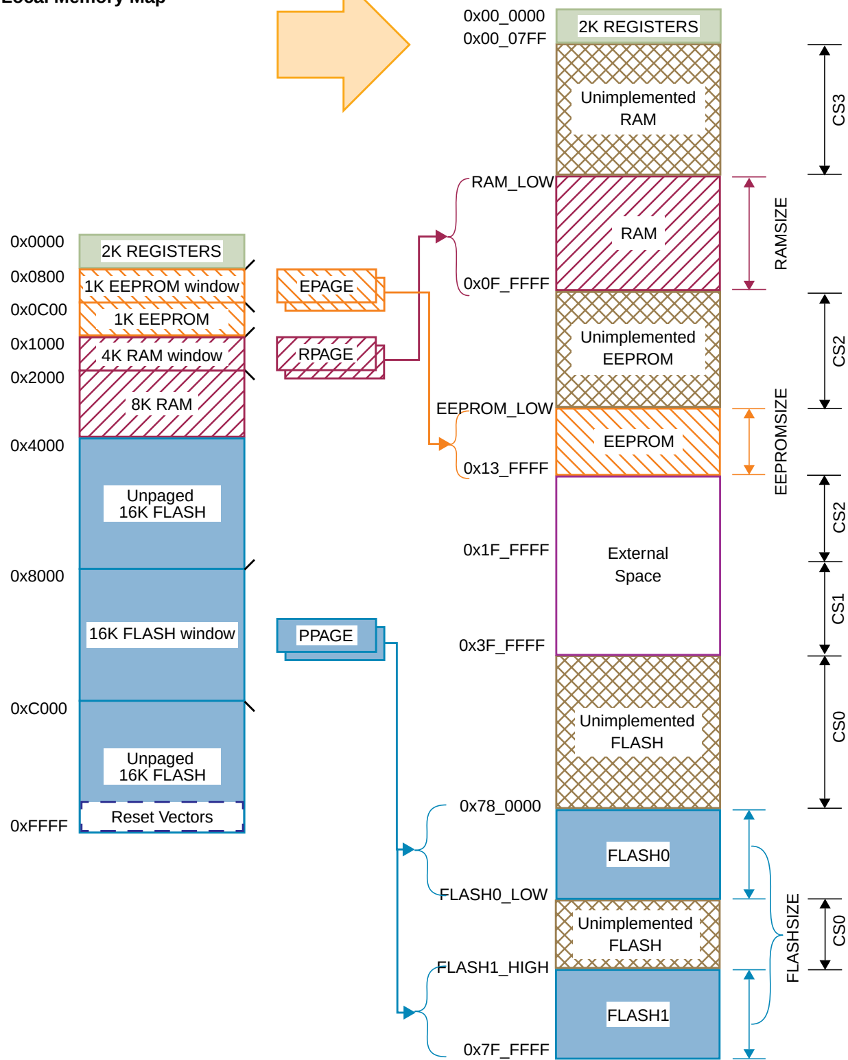
Figure 1-4. S12X CPU & BDM Global Address Mapping
