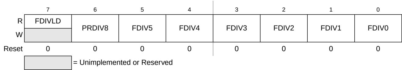
Figure 28-4. Flash Clock Divider Register (FCLKDIV)
