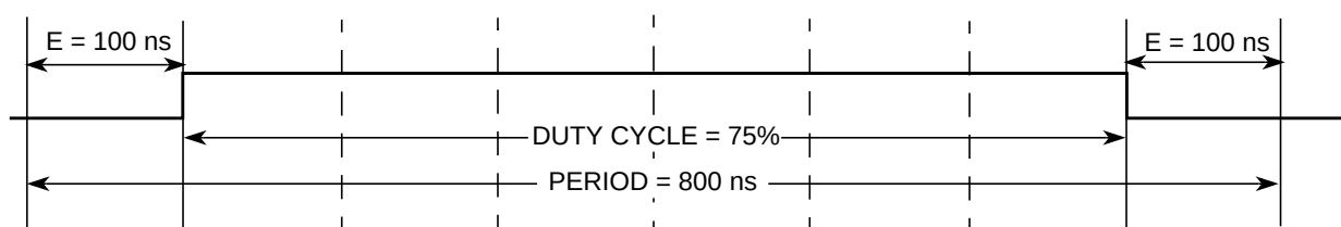
Figure 8-23. PWM Center Aligned Output Example Waveform
