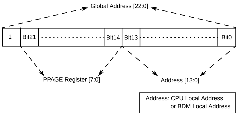
Figure 17-16. PPAGE Address Mapping
