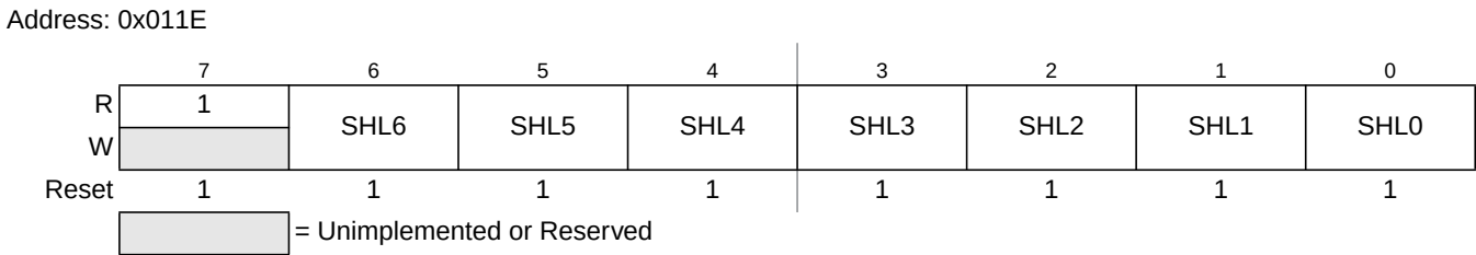
Figure 18-19. RAM Shared Region Lower Boundary Register (RAMSHL)
