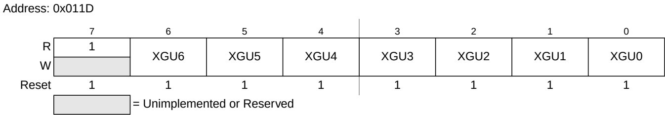
Figure 18-18. RAM XGATE Upper Boundary Register (RAMXGU)
