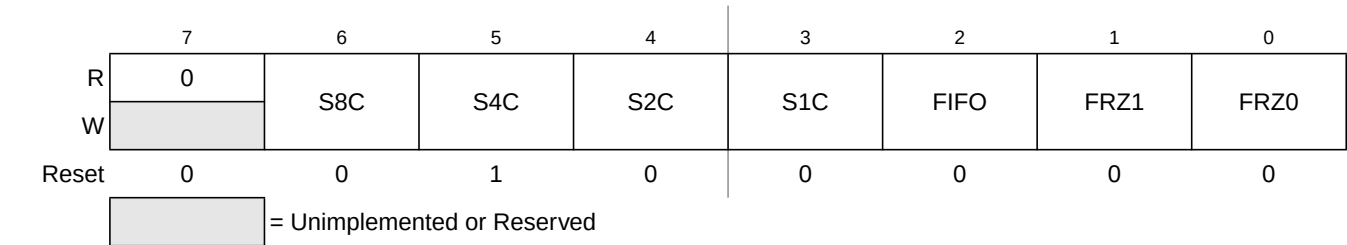
Figure 4-6. ATD Control Register 3 (ATDCTL3)
