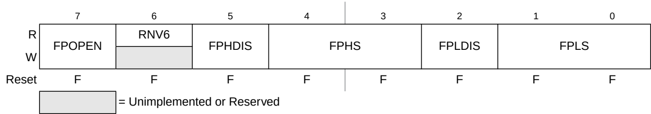
Figure 29-8. Flash Protection Register (FPROT)
