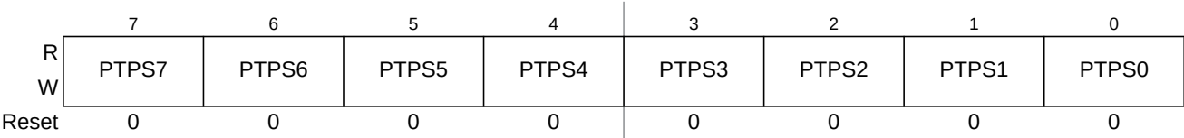
Figure 7-47. Precision Timer Prescaler Select Register (PTPSR)
