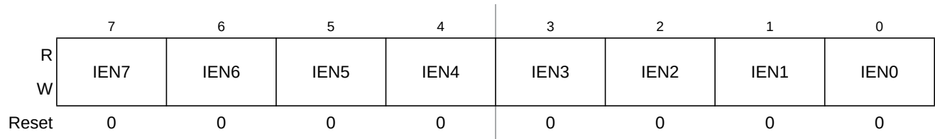
Figure 4-15. ATD Input Enable Register 1 (ATDDIEN1)
