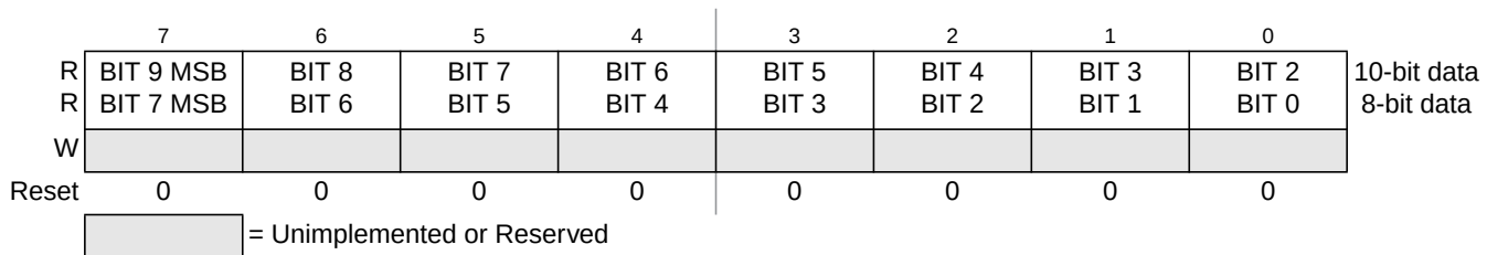
Figure 5-15. Left Justified, ATD Conversion Result Register, High Byte (ATDDRxH)
