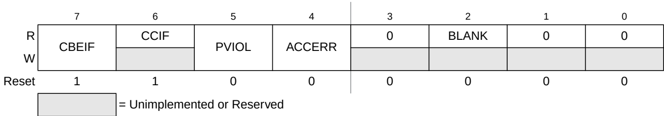
Figure 25-9. EEPROM Status Register (ESTAT — Normal Mode)
