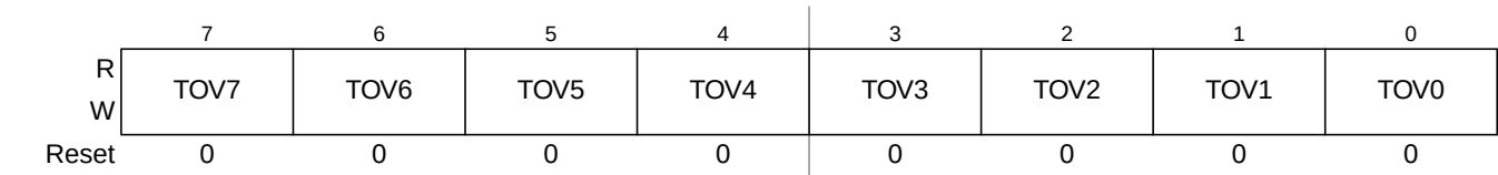
Figure 7-10. Timer Toggle On Overflow Register 1 (TTOV)
