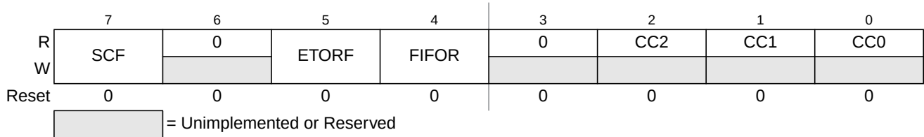
Figure 5-9. ATD Status Register 0 (ATDSTAT0)
