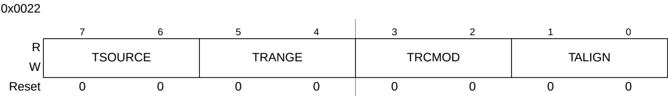
Figure 19-5. Debug Trace Control Register (DBGTCR)
