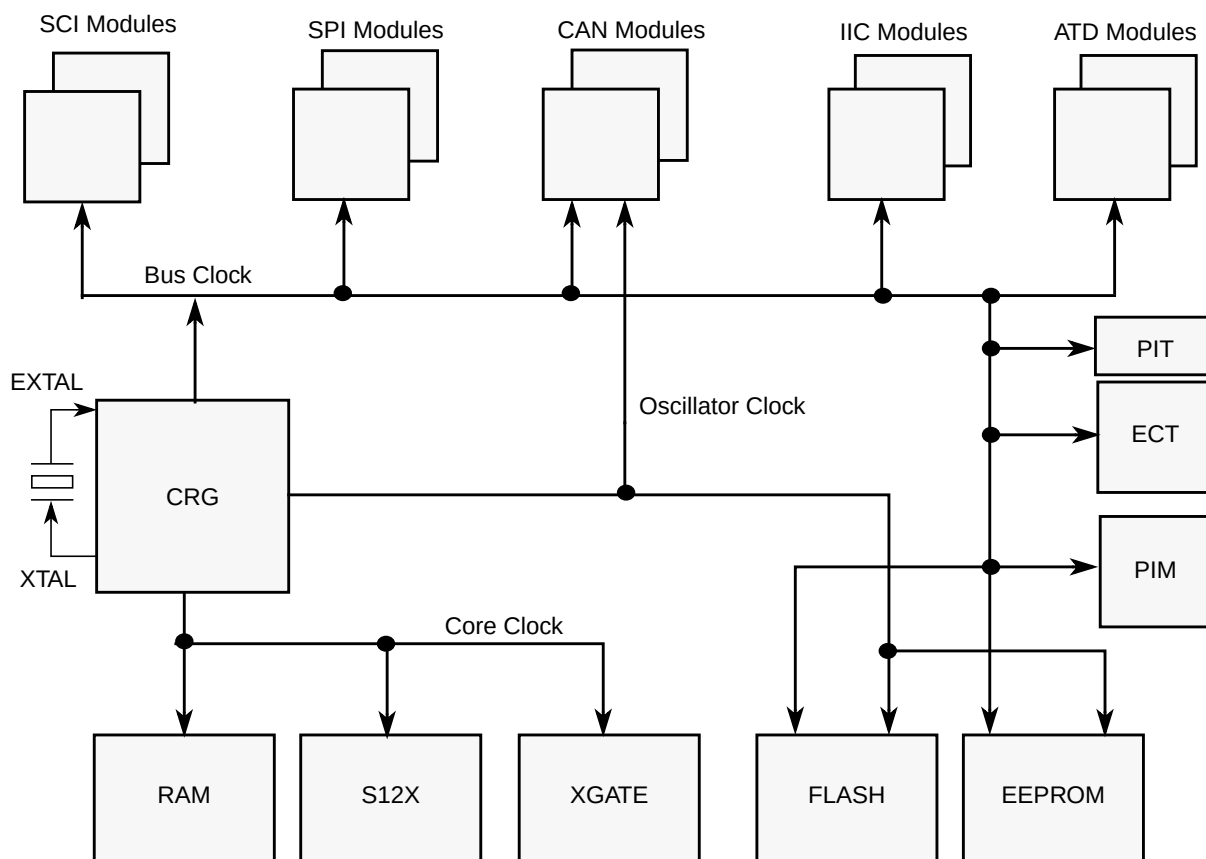
Figure 1-14. MC9S12XD Family Clock Connections
