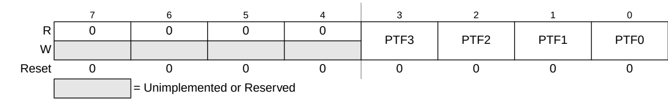
Figure 13-8. PIT Time-Out Flag Register (PITTF)
