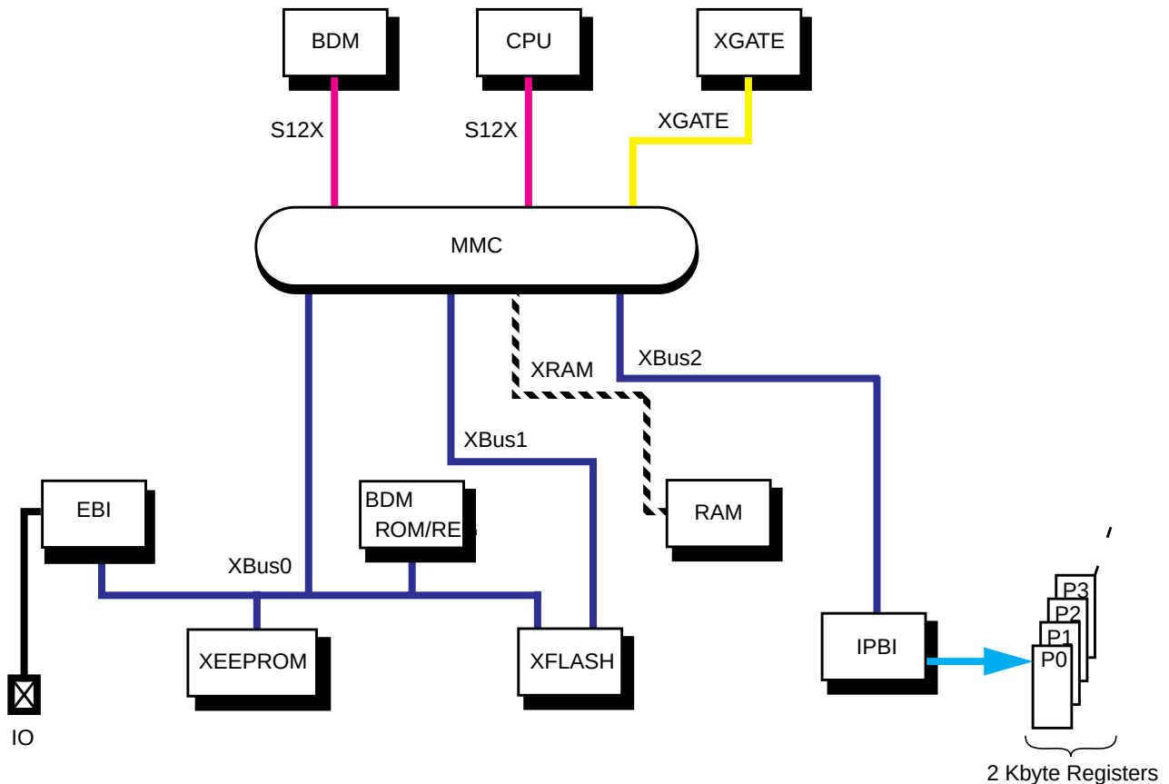
Figure 17-26. S12X Architecture
