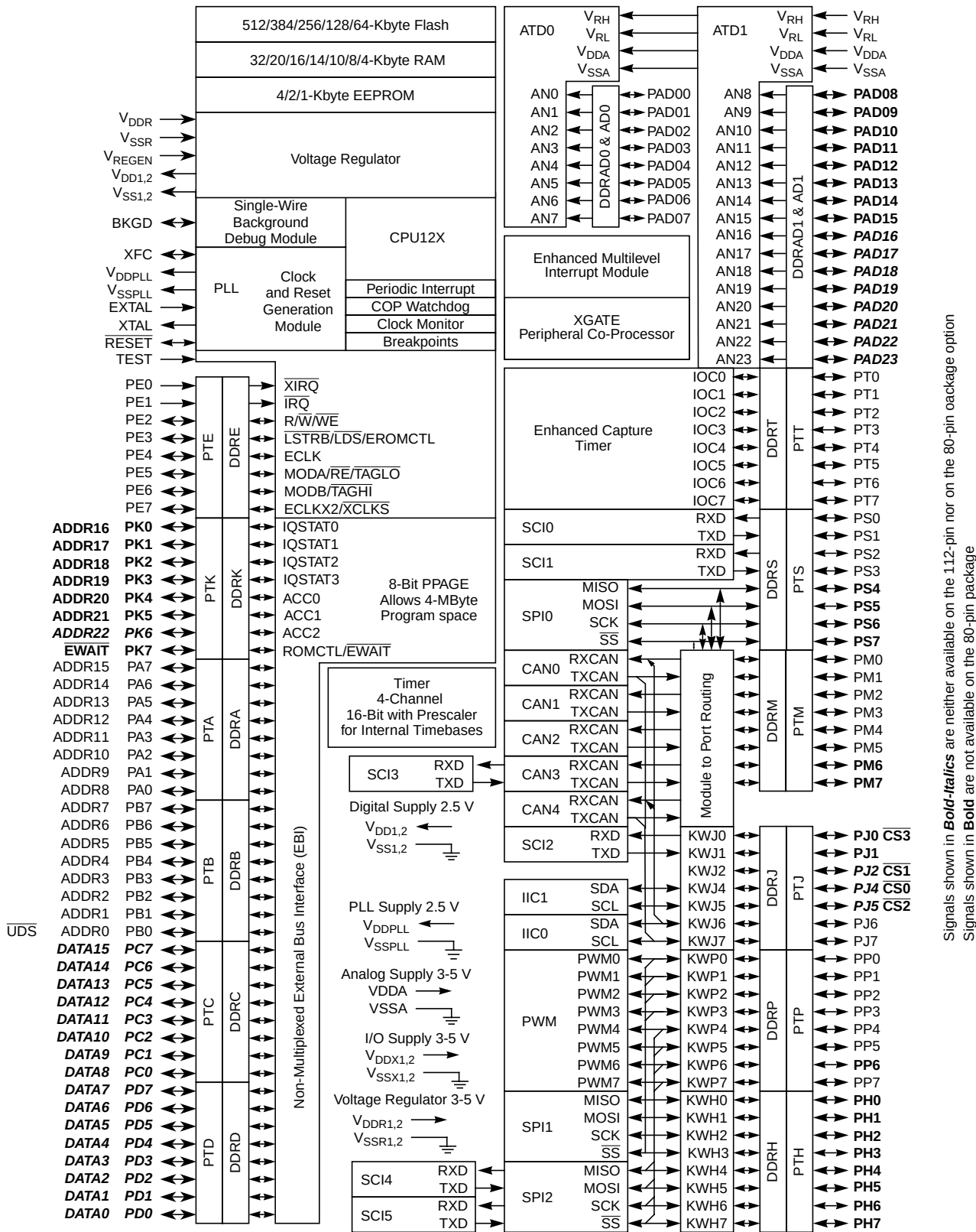
Figure 1-1. MC9S12XD-Family Block Diagram
