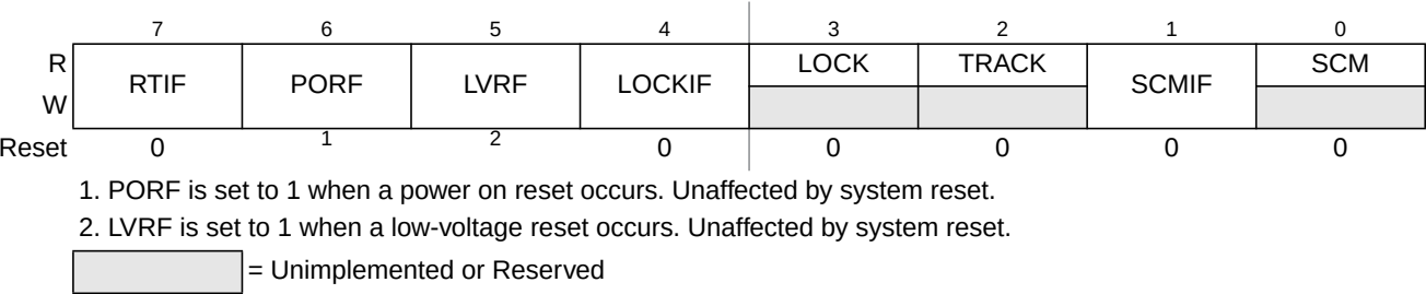
Figure 2-7. CRG Flags Register (CRGFLG)
