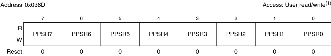
Figure 2-88. Port R Polarity Select Register (PPSR)
