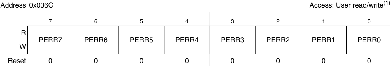
Figure 2-87. Port R Pull Device Enable Register (PERR)
