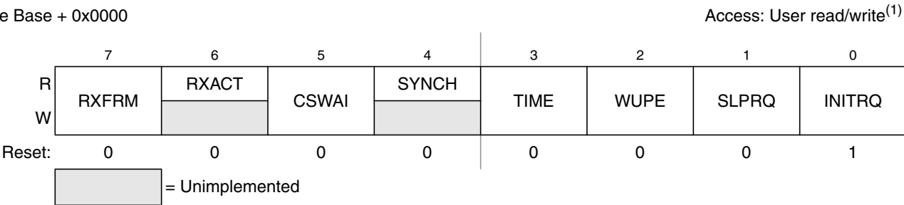
Figure 16-4. MSCAN Control Register 0 (CANCTL0)
