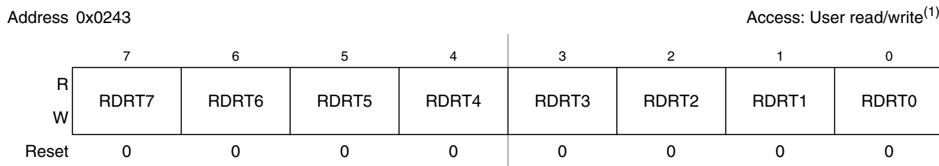
Figure 2-22. Port T Reduced Drive Register (RDRT)
