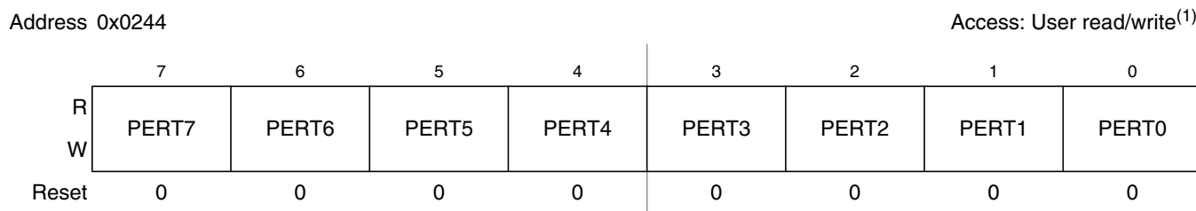
Figure 2-23. Port T Pull Device Enable Register (PERT)
