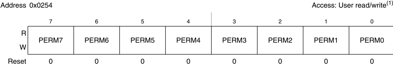
Figure 2-39. Port M Pull Device Enable Register (PERM)
