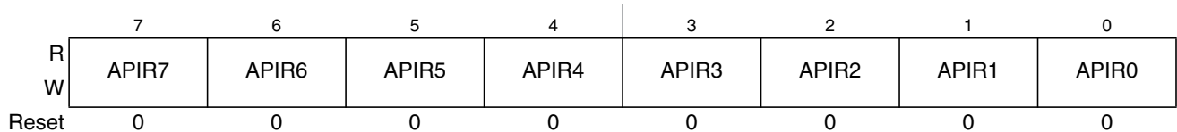
Figure 23-7. Autonomous Periodical Interrupt Rate Low Register (VREGAPIRL)
