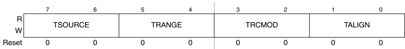
Figure 8-5. Debug Trace Control Register (DBGTCR)
