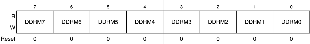
Figure 2-37. Port M Data Direction Register (DDRM)
