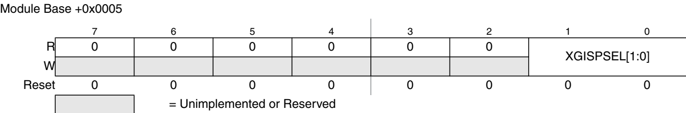
Figure 10-6. XGATE Initial Stack Pointer Select Register (XGISPSEL)
