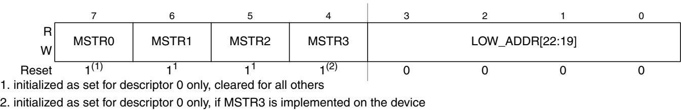
Figure 4-8. MPU Descriptor Register 0 (MPUDESC0)
