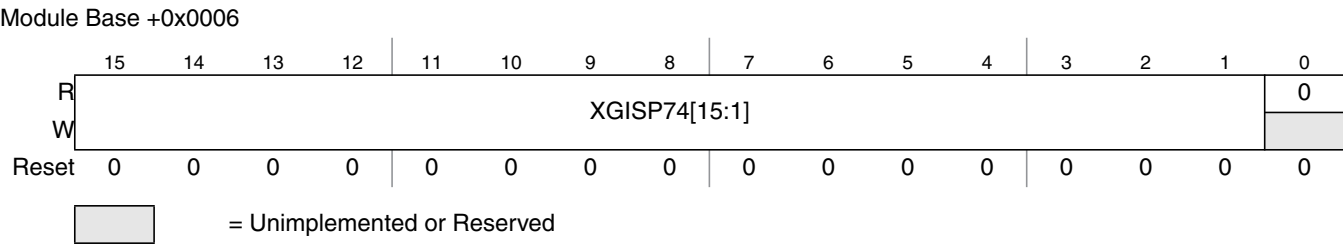
Figure 10-7. XGATE Initial Stack Pointer for Interrupt Priorities 7 to 4 (XGISP74)
