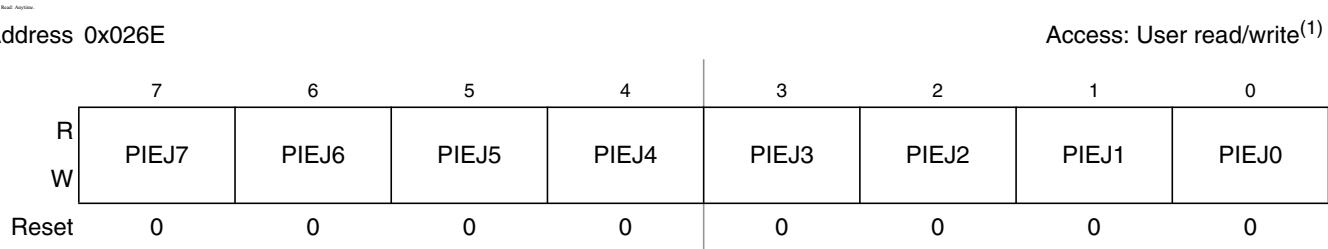
Figure 2-65. Port J Interrupt Enable Register (PIEJ)
