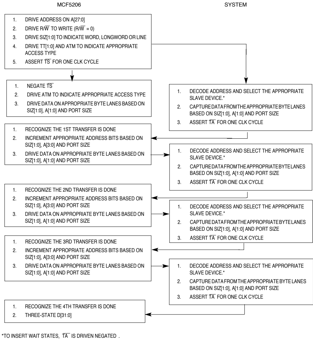
Figure 6-10. Word-, Longword-, and Line-Write Transfer Flowchart
