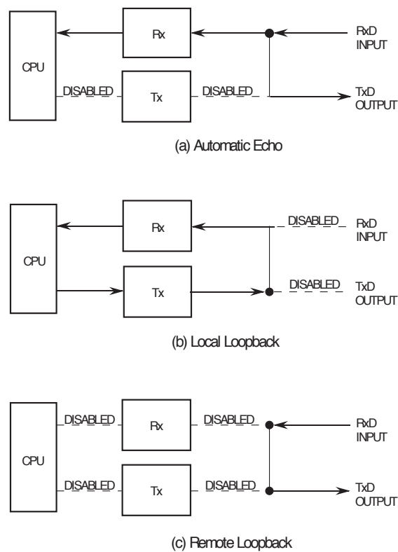
Figure 11-7. Looping Modes Functional Diagram
