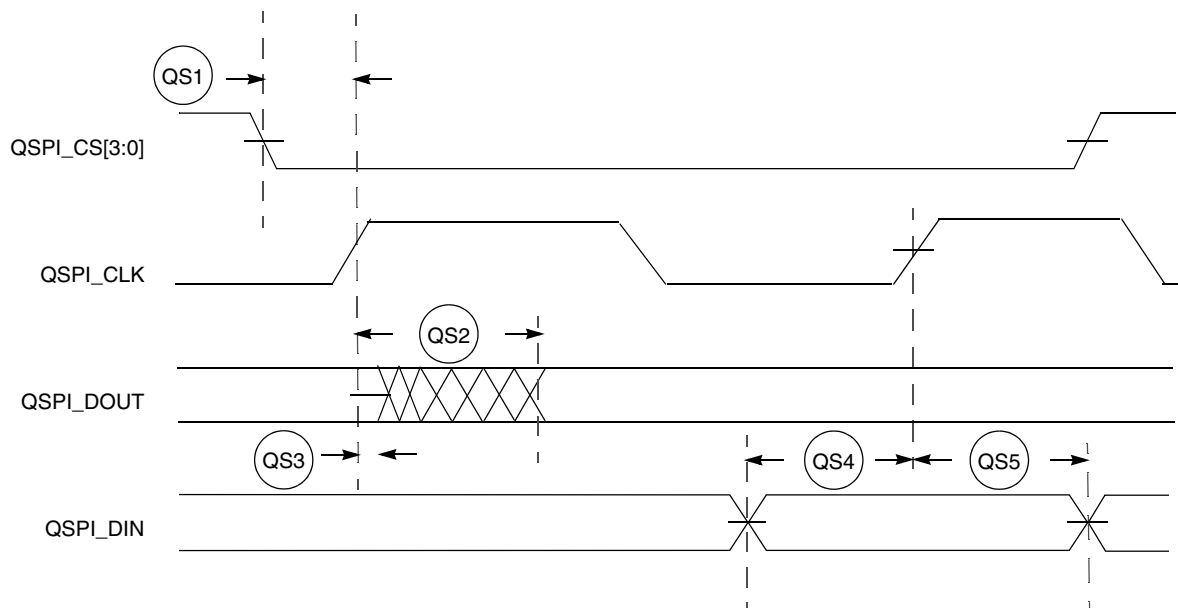
Figure 13. QSPI Timing
