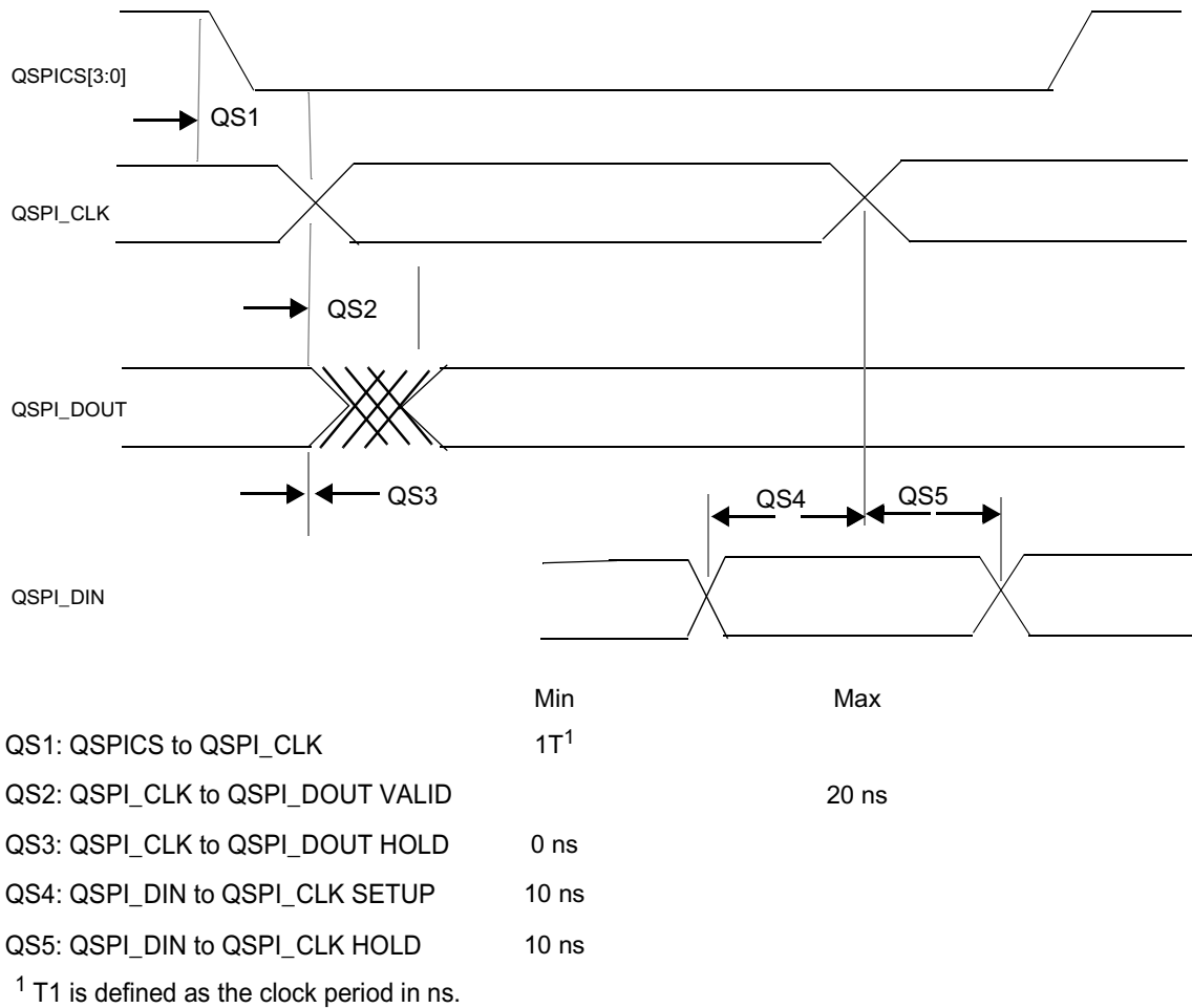
Figure 16-11 QSPI Timing
