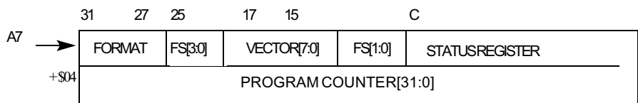
Figure 3-5 Exception Stack Frame Form
