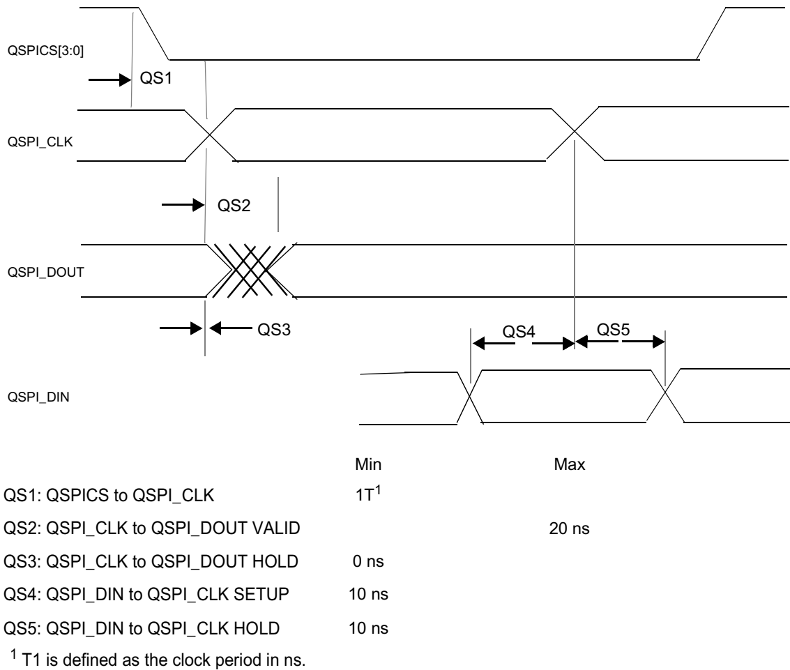
Figure 16-11 QSPI Timing
