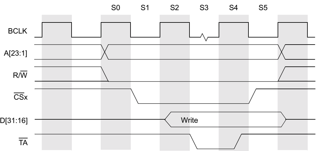
Figure 8-6 Basic Write Bus Cycle
