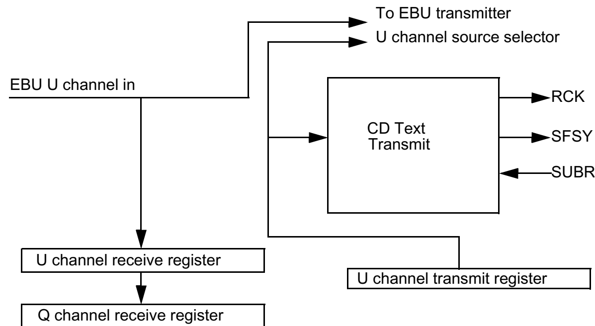
Figure 17-4 CD-Subcode Interface
