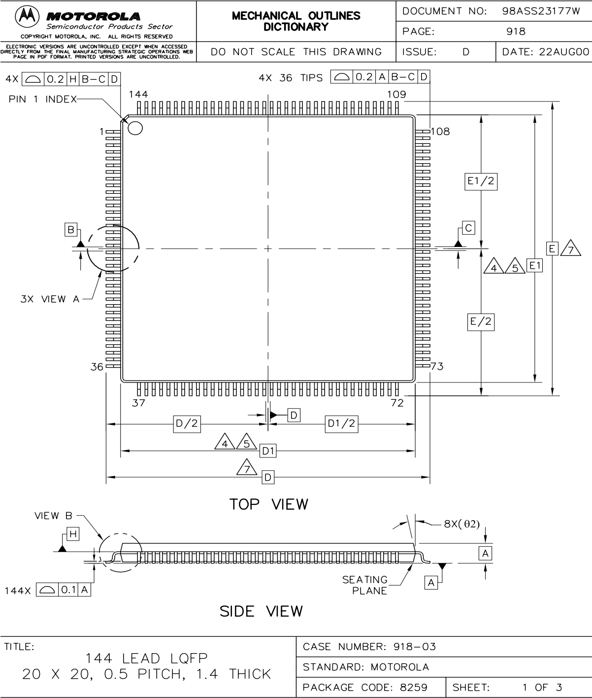
Figure 22-1 144 QFP Package (1 of 3)
