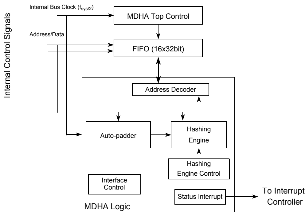
Figure 26-11. MDHA Block Diagram
