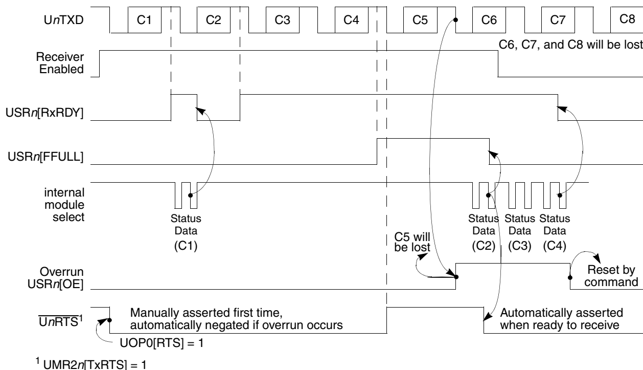
Figure 24-20. Receiver Timing
