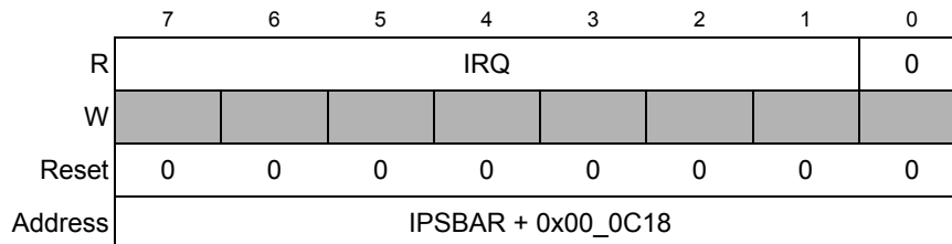
Figure 13-7. Interrupt Request Level Register (IRLR)
