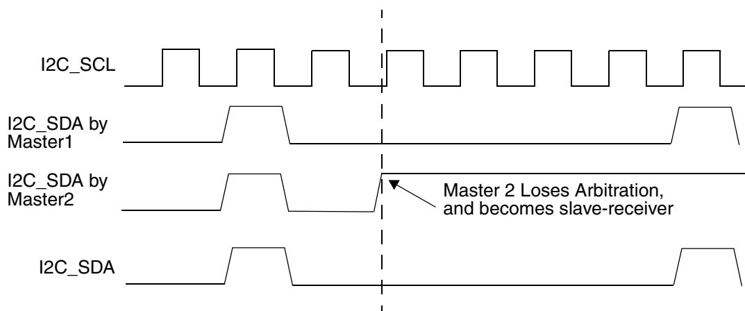
Figure 25-7. Arbitration Procedure
