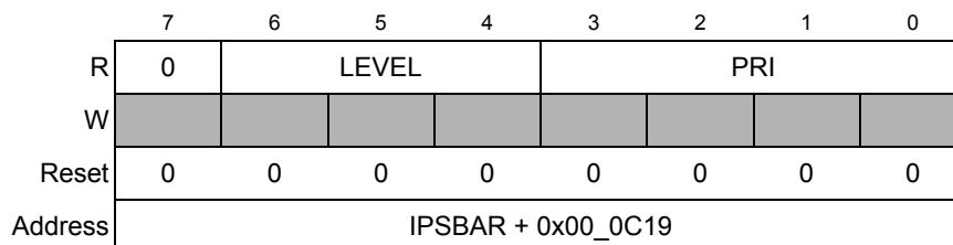
Figure 13-8. IACK Level and Priority Register (IACKLPR)
