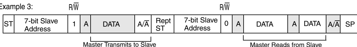
Figure 25-6. Data Transfer, Combined Format
