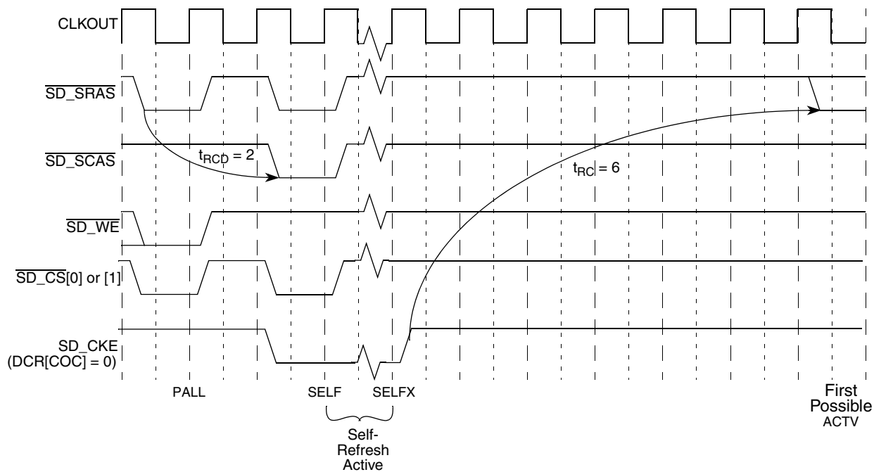
Figure 18-9. Self-Refresh Operation
