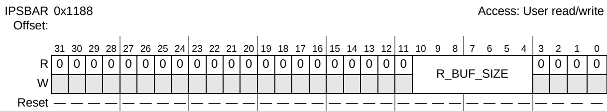
Figure 17-24. Receive Buffer Size Register (EMRBR)
